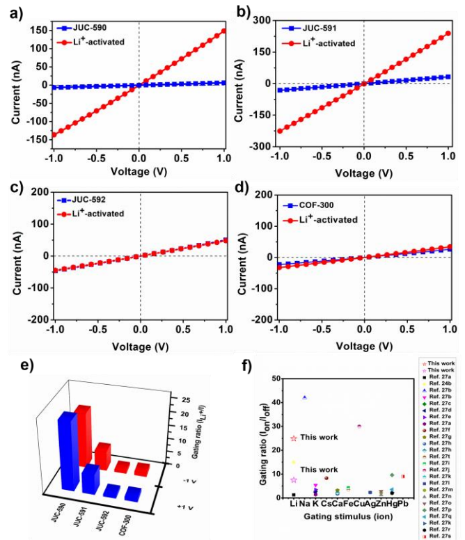
Figure 2. I-V curves of JUC-590-MMM (a), JUC-591-MMM (b), JUC-592-MMM (c), and COF-300-MMM (d) before (blue square) and after (red circle) activation with \text{Li}^+ . (e) The gating ratio ( I_{\text{on}}/I_{\text{off}} ) of JUC-590-, JUC-591-, JUC-592- and COF-300-MMM at -1 \text{ V} and +1 \text{ V} . (f) Comparison of the gating ratios of 3D functionalized COFs and other reported 1D nanochannels activated by metal ions.
