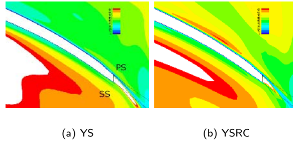
FIG. 4: Trailing-edge close up of a 10 % span blade-to-blade view of the field of the normalized turbulent viscosity \mu_t/\mu . Contrary to the blade-to-blade midspan of figure 3, here the YSRC correction reproduces the effect of rotation: turbulence is increased close to pressure side at the trailing edge.
