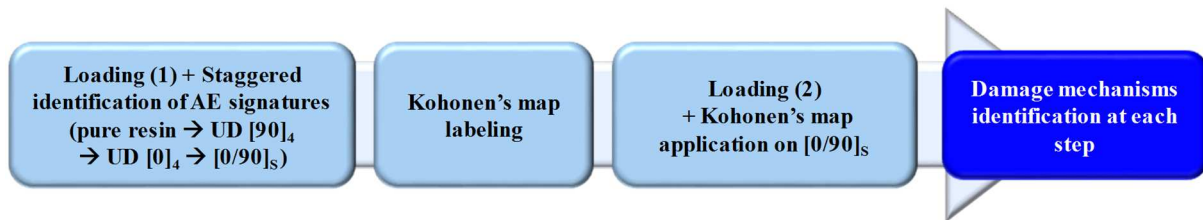
Fig.5. Adopted approach during the two mechanical loadings (1) & (2).
