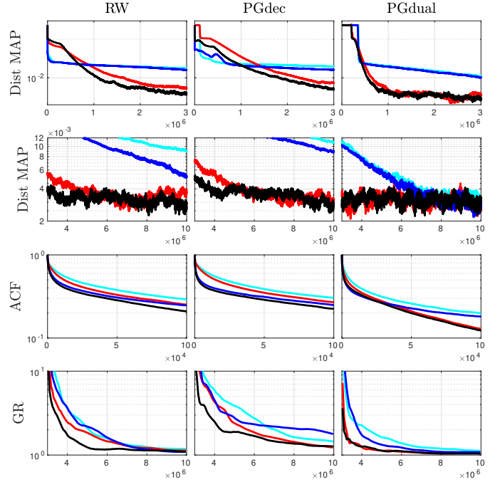
Fig. 1: Displayed: the normalized distance to \hat{\mathbf{R}}_{\text{MAP}} versus the iteration index, during the burn-in phase (row 1) and after the burn-in phase (row 2); the ACF criterion versus the lag (row 3) and the GR criterion versus the iteration index (row 4); for the RW-based samplers (column 1), PGdec-based samplers (column 2) and PGdual-based samplers (column 3). For each Algo in \{\text{RW, PGdec, PGdual}\} : Algo I is in cyan, Algo O is in red, Gibbs Algo I is in blue and Gibbs Algo O is in black.
