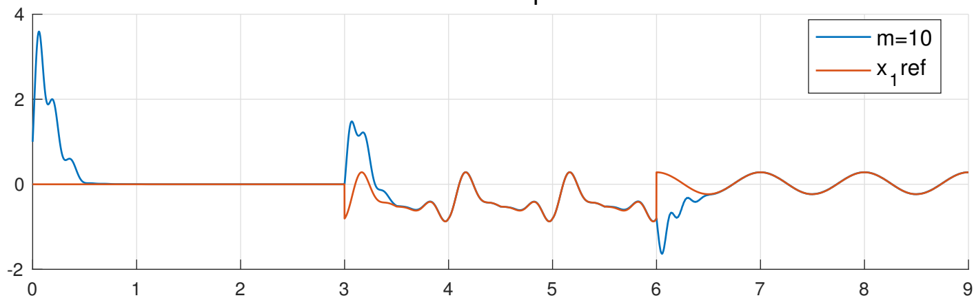
State x_1
