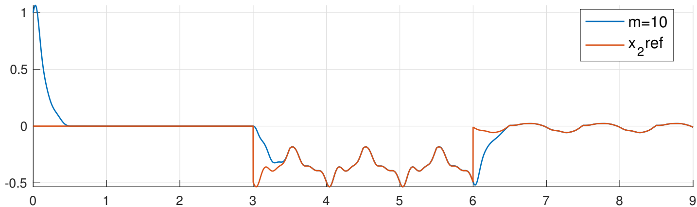
State x_2
