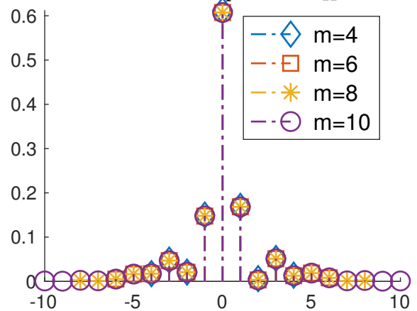
Modulus of phasors \tilde{P}_{22}
