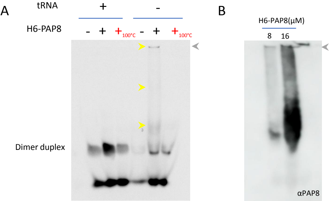
Figure S2. (A) rEMSA gel: 5% polyacrylamide 29:1 in 1X TBE running buffer. +100 ° C, boiled PAP8 sample; yellow arrowheads, probe shift. (B) Western blot using PAP8 antiserum on the rEMSA native gel. Gray arrowheads, position of the wells.
