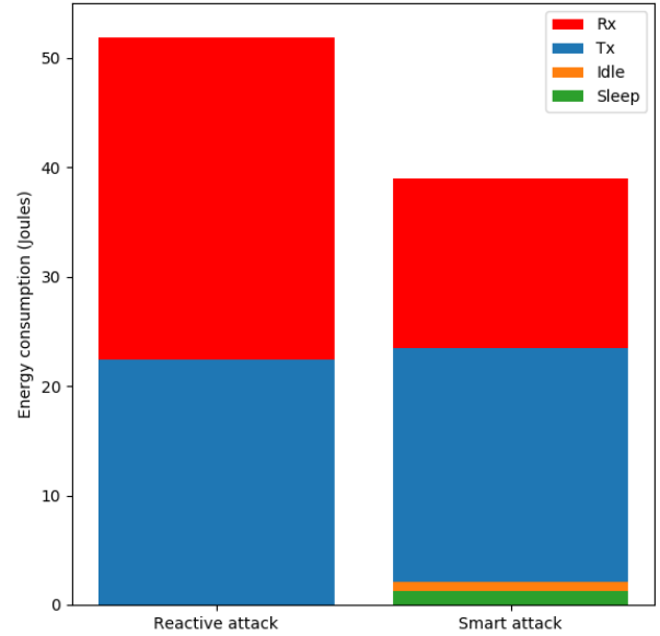
Fig. 4: Comparison of energy consumption between reactive and smart attack.
