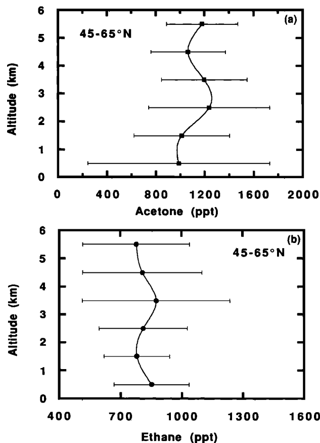
Fig. 3. Mean vertical structure of (a) acetone and (b) ethane. Horizontal bars show one standard deviation.
