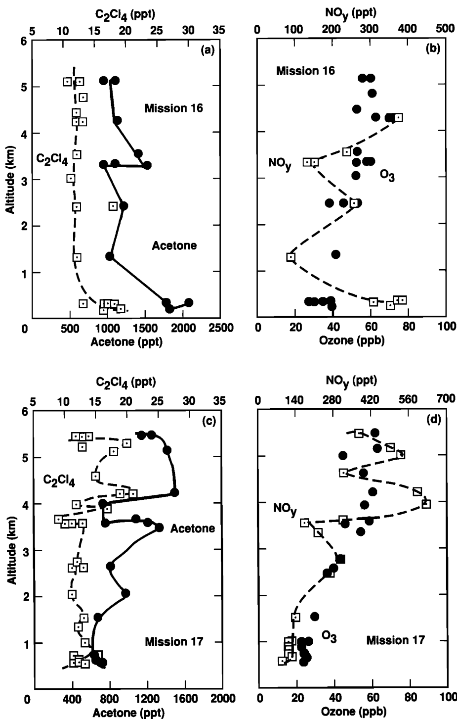
Fig. 10. (a and b) Evidence for acetone enhancement within a polluted air mass in the boundary layer (mission 16, August 9, 1990) and (c and d) the free troposphere (mission 17, August 11, 1990). C 2 Cl 4 , O 3 , and NO y distributions are also shown.
