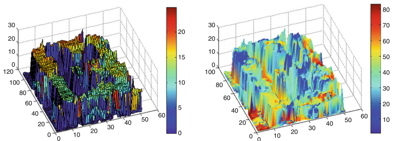
Fig. 5.31 3-D tomographic reconstruction using dual-baseline PolInSAR data sets, shaded by surface elevation (left) and \alpha value (right)
