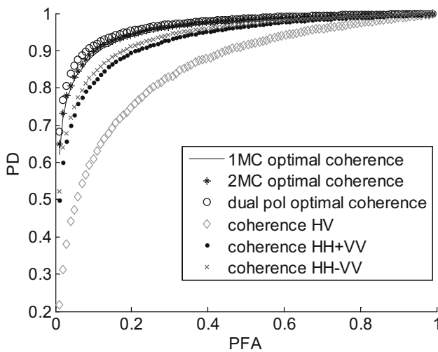
Fig. 5.19 ROC: Benefit of a coherence optimization
