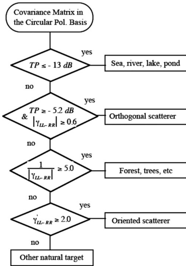
Fig. 5.7 Classification algorithm
