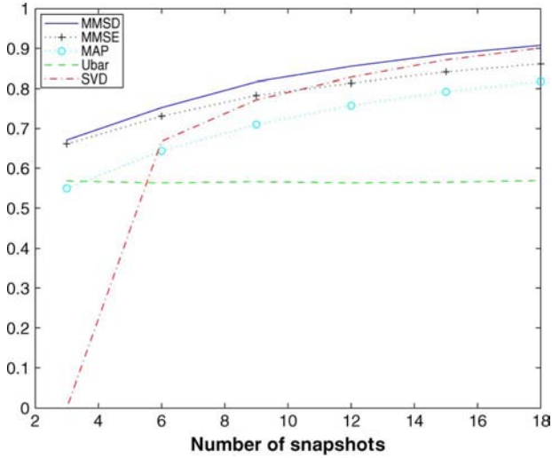
Fig. 6. Fraction of energy of \hat{U} in \mathcal{R}(\mathbf{U}) versus K . N = 20 , p = 5 , \kappa = 20 , and SNR = 5 dB. Linear model, vMF prior.
