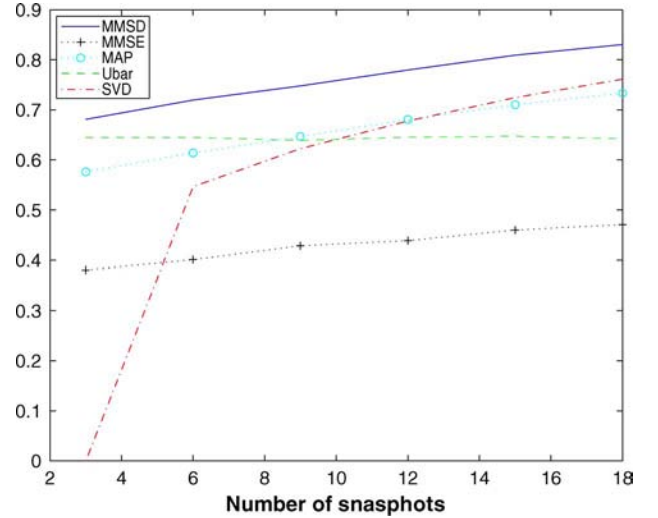
Fig. 8. Fraction of energy of \hat{U} in \mathcal{R}(\mathbf{U}) versus K . N = 20 , p = 5 , \kappa = 20 , SNR_- = 5 dB, and SNR_+ = 10 dB. Covariance matrix model, Bingham prior.
