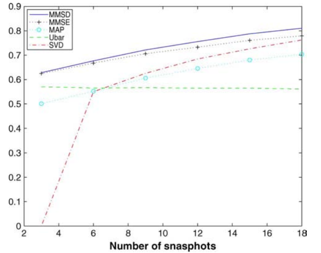
Fig. 9. Fraction of energy of \hat{U} in \mathcal{R}(\mathbf{U}) versus K . N = 20 , p = 5 , \kappa = 20 , SNR_- = 5 dB, and SNR_+ = 10 dB. Covariance matrix model, vMF prior.
