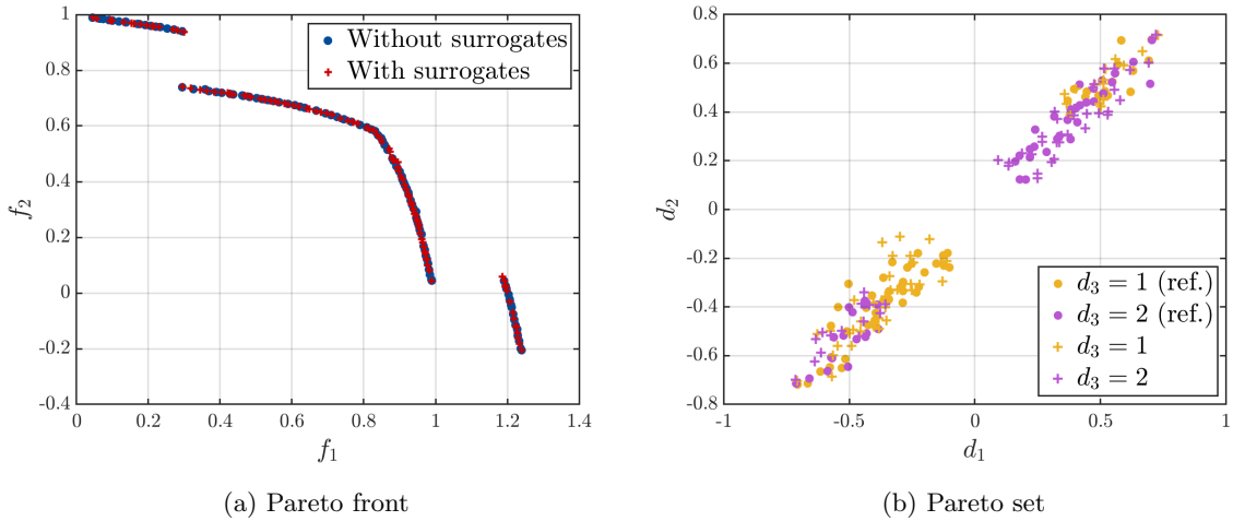
Figure 11: Example 2: Comparison of the Pareto fronts and sets for the results with median relative hypervolume error and the reference solution.
