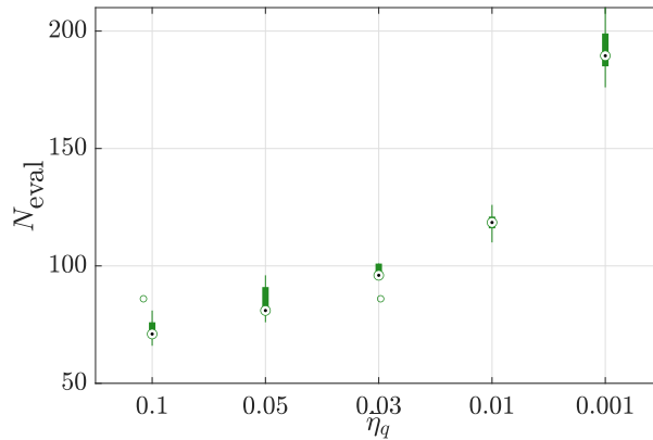
Figure 5: Example 1: Number of model evaluations for various thresholds of the stopping criterion.
