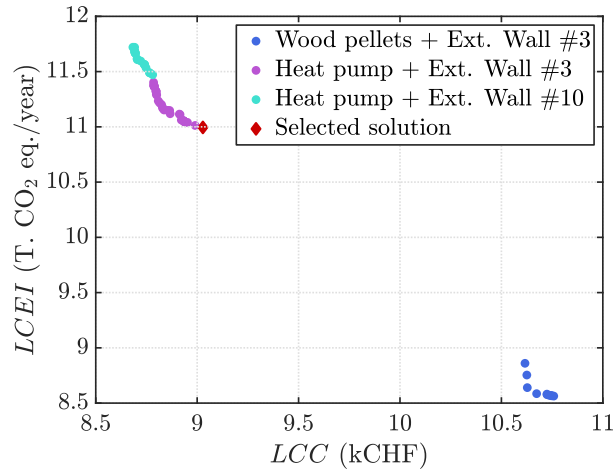
Figure 14: Example 3: Pareto front and selected solution.
