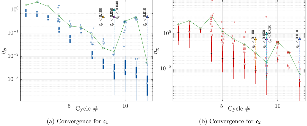
Figure 10: Example 2: Relative error of the quantiles of the costs \mathbf{c}_1 and \mathbf{c}_2 for the entire Pareto front at the end of each cycle. The upper convergence limit is shown by the continuous line.
