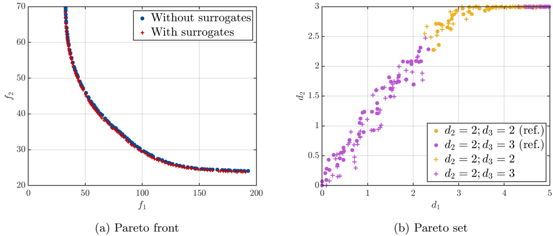
Figure 7: Example 1: Comparison of the Pareto fronts and sets for the results with median relative hypervolume error and the reference solution.
