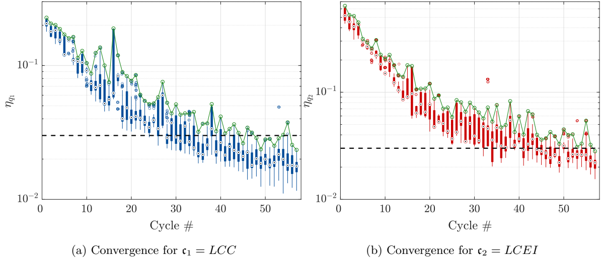
Figure 13: Example 3: Relative quantile error of the entire Pareto front at the end of each cycle.
