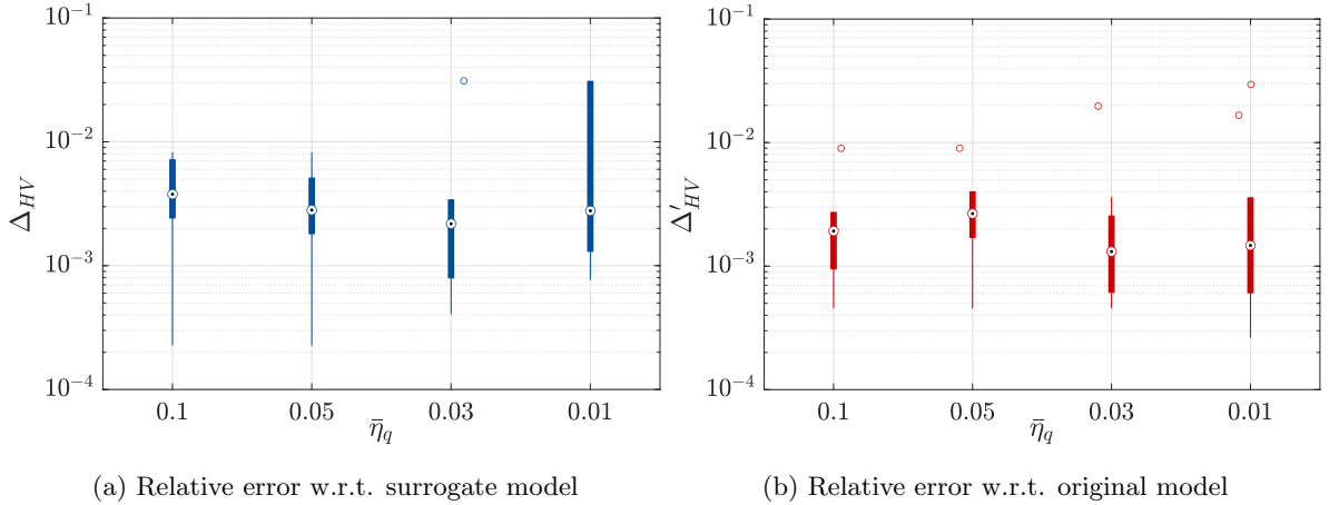
Figure 8: Example 2: Relative errors w.r.t. the reference hypervolume for various thresholds of the stopping criterion.
