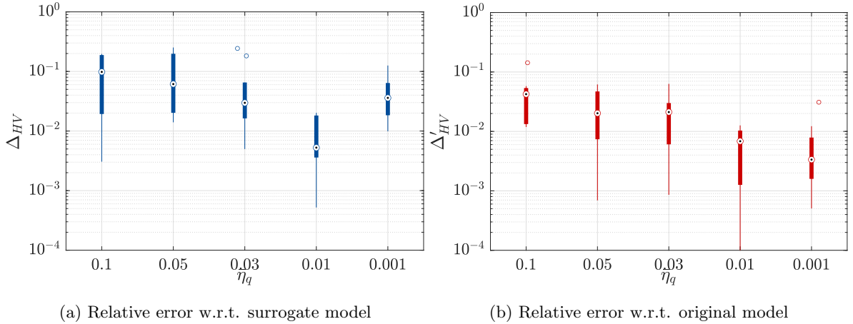
Figure 4: Example 1: Relative errors w.r.t. the reference hypervolume for various thresholds of the stopping criterion.
