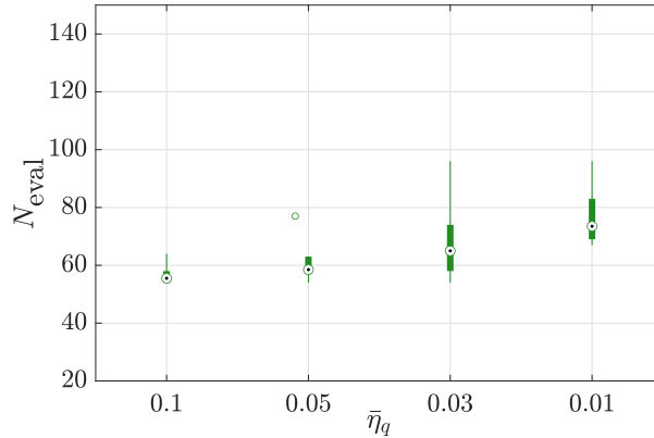
Figure 9: Example 2: Number of model evaluations for various thresholds of the stopping criterion.
