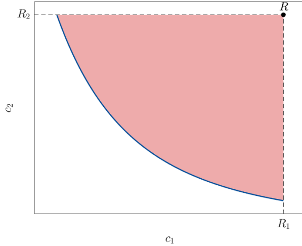
Figure 3: Illustration of the hypervolume as the red shaded area. The reference Pareto front \mathcal{F}_{\text{ref}} is represented by the blue line while the Nadir point R is shown by the black dot.
