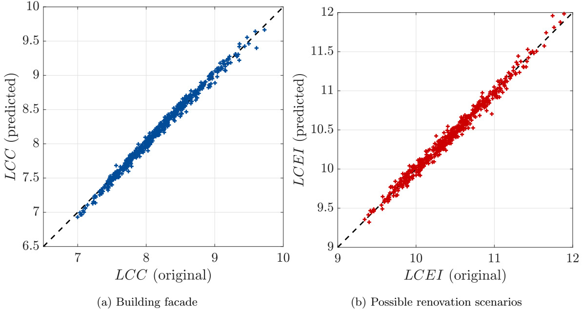
Figure 15: Example 3: Original vs. predicted responses for a subset of the Monte Carlo set used to compute the quantiles at the selected solution.
