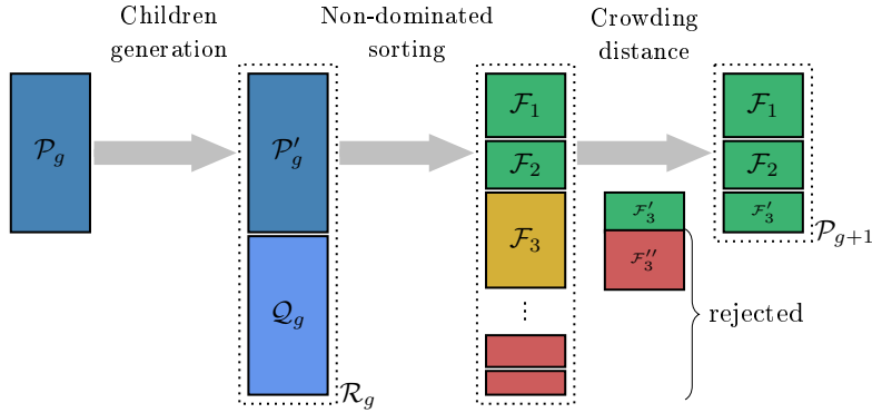
Figure 1: Flowchart of NSGA-II (adapted from Deb et al. (2002)).
