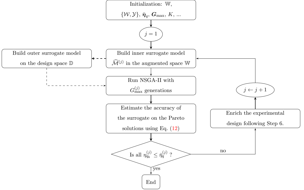
Figure 2: Flowchart of the proposed approach.
