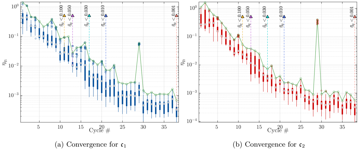
Figure 6: Example 1: Relative error of the 90% quantiles of the costs \mathbf{c}_1 and \mathbf{c}_2 for the entire Pareto front at the end of each cycle. The upper convergence limit is shown by the continuous line.
