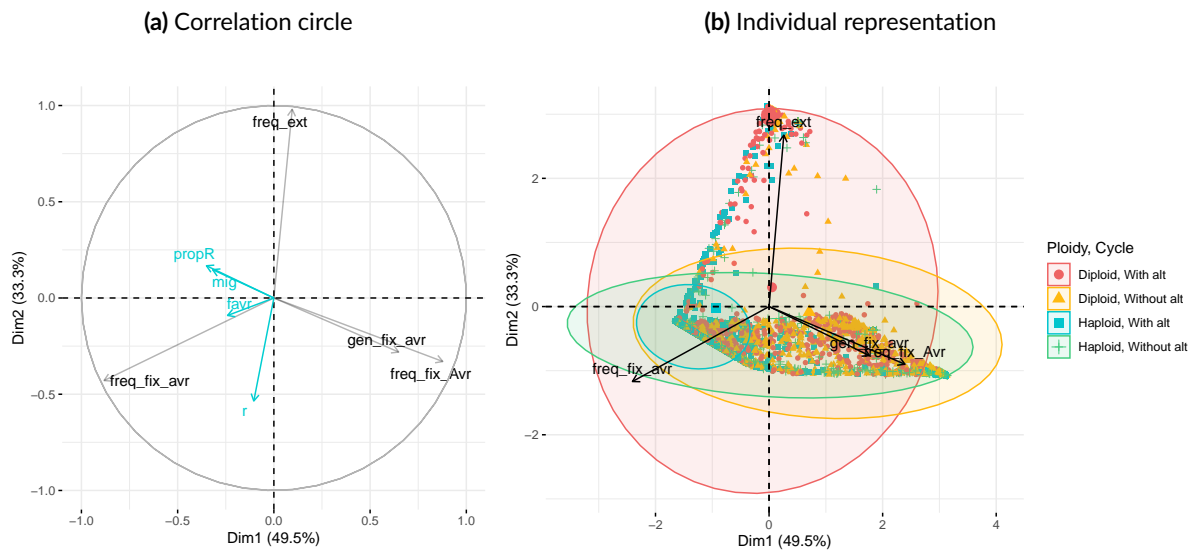
Figure 2 – Principal component analysis on four output variables: freq_ext , freq_fix_Avr , freq_fix_avr , and gen_fix_avr . Two results are displayed: (a) the correlation circle on four output variables. The quantitative parameters f_{avr} , mig , r , and propR are represented informatively in blue on the correlation circle and do not contribute to the variability; (b) the individual representation of simulations which represents the influence of the pathogen ploidy and life cycle. Each point represents a different combination of parameters with 100 replicates. Ellipses correspond to the 95% multivariate distribution.
