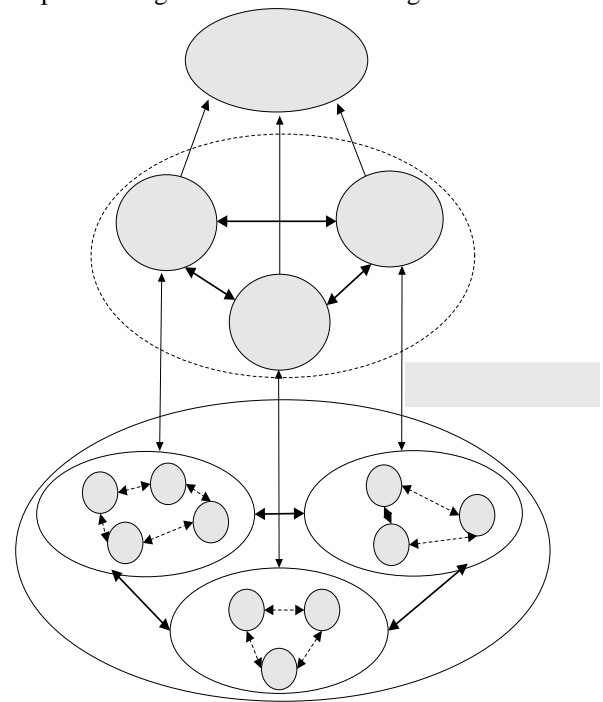
Figure 5: Multi-Agent Architecture.
