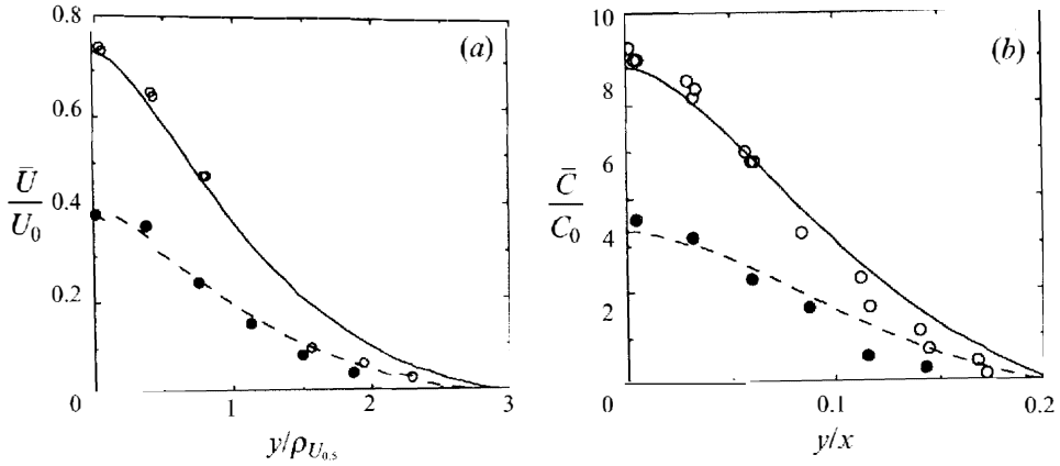
FIGURE 10. Heavy jet: (a) mean axial velocity and (b) mean mass-fraction profiles across the jet. x/R_0 = 20 : \circ , Exp. C79; —, model. x/R_0 = 40 : \bullet , Exp. C79; - - -, model.
