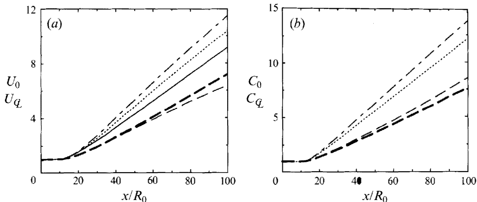
FIGURE 13. Decay of centreline mean velocity (a) and centerline mean mass-fraction (b) for different density ratios: \cdots , S = 0.57 ; --- , S = 0.7 ; --- , S = 1.0 ; --- , S = 1.43 and g = 9.81 \text{ m s}^{-2} ; --- , S = 1.43 and g = 0 .
