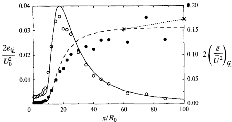
FIGURE 4. Constant-density jet: turbulent kinetic energy along the jet axis. 2\bar{e}_G/U_0^2 : \circ , Exp. C79; —, model. 2(\bar{e}/\bar{U}^2)_G : \bullet , Exp. C79; --, model; *, Wygnanski & Fiedler (1969).
