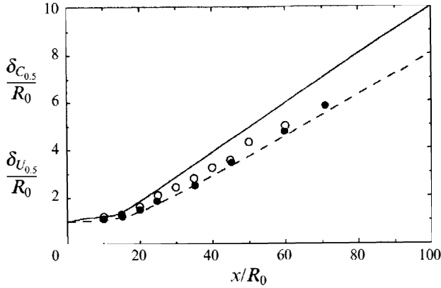
FIGURE 7. Heavy jet: streamwise variations of half-width velocity and mass fraction. \delta_{C_{0.5}}/R_0 : \circ , Exp. C79; —, model. \delta_{U_{0.5}}/R_0 : \bullet , Exp. C79; - - , model.
