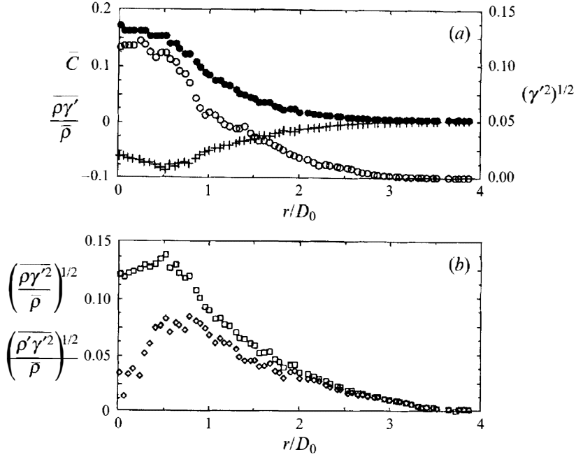
FIGURE 1. (a) \bullet , Mean mass fraction ( \bar{C} ); +, first-order density–mass fraction correlation ( \overline{\rho\gamma'}/\bar{\rho} ); and \circ , mean mass fraction variance (\gamma'^2)^{1/2} in a pure hydrogen–air jet, from Sautet’s measurements (1992). (b) Corresponding profiles of \square , (\overline{\rho\gamma'^2}/\bar{\rho})^{1/2} according to (2.6); and \circ , (\overline{\rho'\gamma'^2}/\bar{\rho}')^{1/2} according to (3.7).
