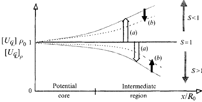
FIGURE 21. Density ratio effects on the mean velocity decay rate near the exit: (a) turbulent diffusion and (b) d.f.c. terms.
