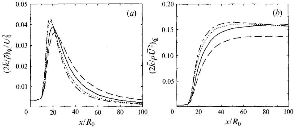
FIGURE 15. Turbulent kinetic energy along the jet axis for different inlet density ratios: (a) 2(\bar{k}/\bar{\rho})_{\mathcal{G}}/U_0^2 ; (b) 2(\bar{k}/\bar{\rho}\bar{U}^2)_{\mathcal{G}} . Same symbols as in figure 13.
