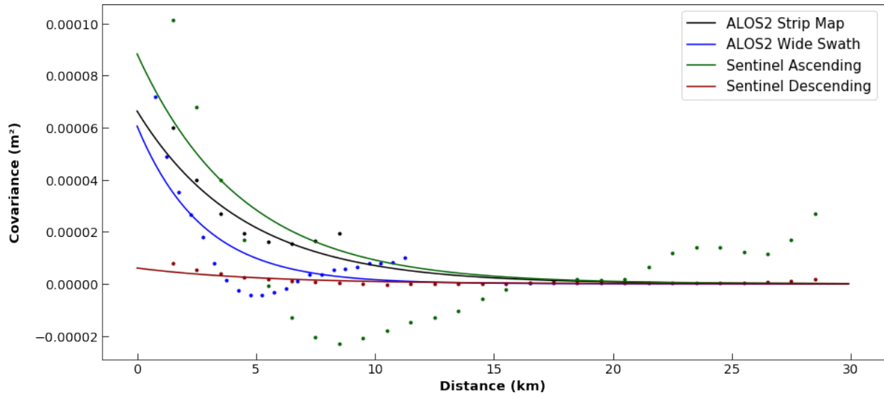
Figure S13. Empirical (dots) and modelled (lines) covariances for the four coseismic interferograms used in the slip inversions.
