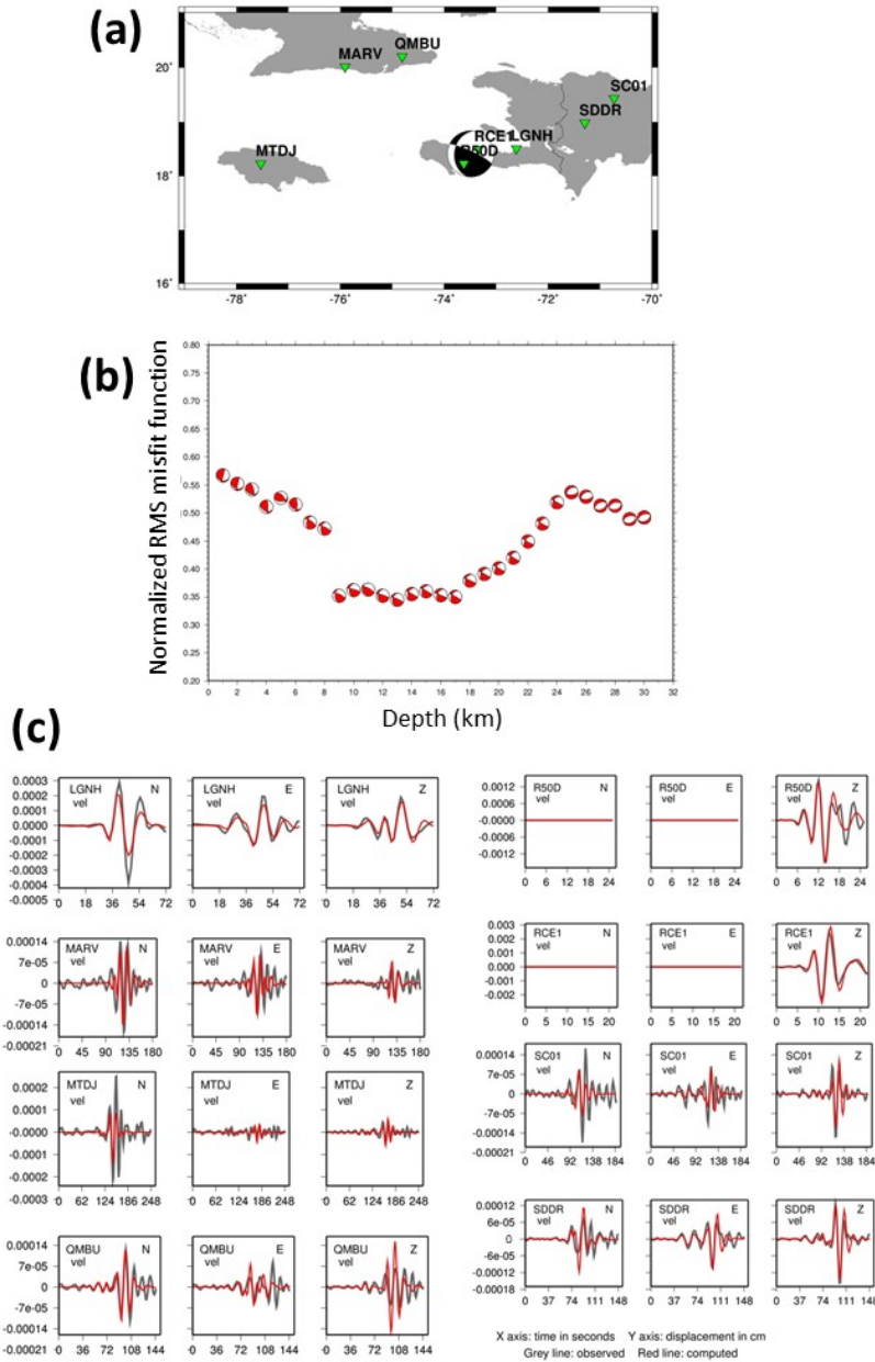
5 Figure S2. Result of the FMNEAR inversion for the 2021/04/06 M14.6 foreshock. (a) Map of stations used (green triangles), with the best solution for the focal mechanism (FM) at its epicentral location. (b) FM solutions as a function of depth and normalized RMS misfit function. The best solution is found at a depth of 13 km, but similar quality solutions are found between 8 and 17km depth. (c) Waveform fit, in displacement (cm) bandpass filtered (see text). Observed records are in gray and computed in red. For each station the three components are displayed (N, E, Z), and ‘vel’ or ‘acc’ means that the original record was in velocity (broadband) or in acceleration (strong motion), respectively. Station names may be truncated if they contain more than four letters. In the case of RS stations R50D4 and RCE1F, only the vertical (Z) component is used, and the N and E velocimetric components, not existing, are shown as flat. 10
