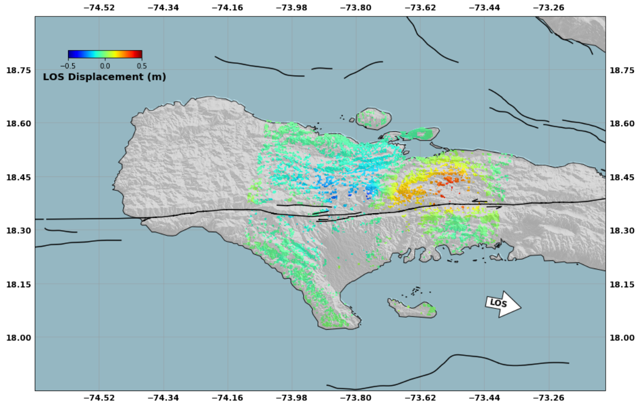
Figure S12. Displacement along the direction of the Line-Of-Sight computed from the interferogram formed of ALOS-2 acquisitions in wide-swath mode along a descending track on December 10, 2019 and August 17, 2021. Black lines are mapped faults from (24). Background shading is topography from SRTM ( Error! Reference source not found. ). White arrow is the surface projection of the LOS direction pointing toward the satellite. Positive motion is toward the satellite. We only use swath 5 which covers the rupture.
