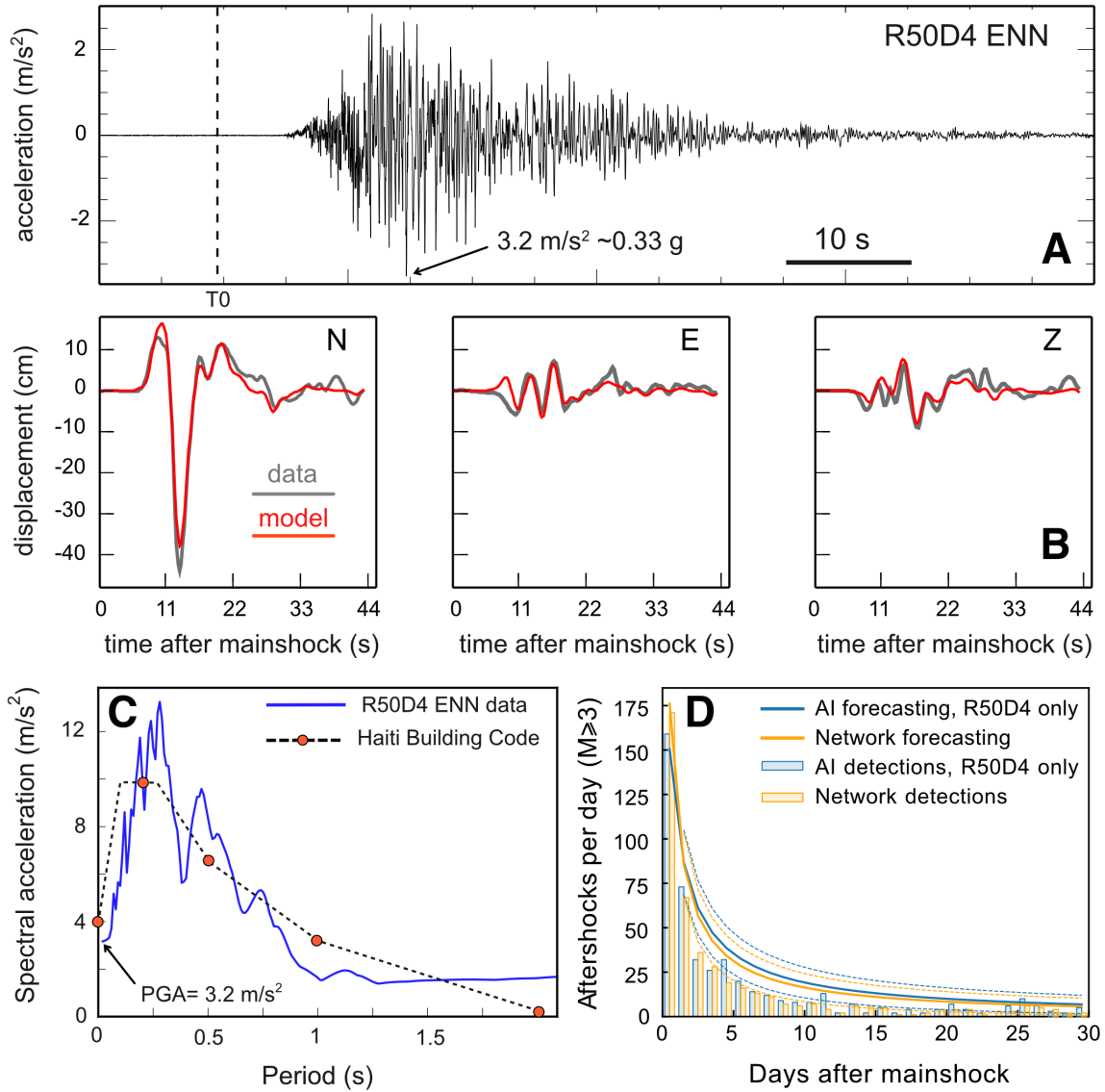
Fig. 2. Data and inferences from citizen station R50D4, 21 km from the 2021 Nippes earthquake
