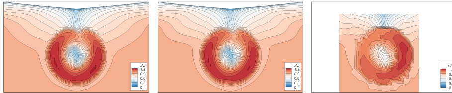
Figure 18: KCS self-propulsion: axial velocity in the propeller plane x/L = 0.9911 . Left to right: T_{\tau H} = 0.1L , 0.025L , and experiments.
