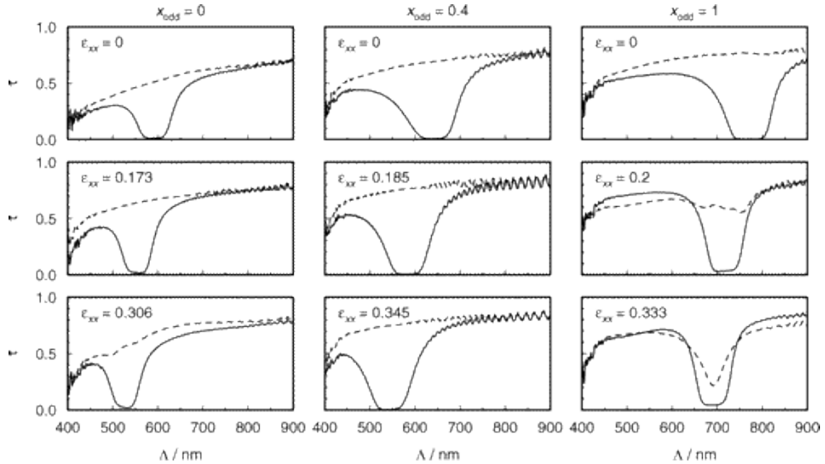
Figure 5 Transmission spectra of three elastomers with different relative molar fractions x_{\text{odd}} for left (solid curves) and right circularly polarized light (dashed curves) at room temperature for different uniaxial strains \epsilon_{xx} perpendicular to the helical axis.
