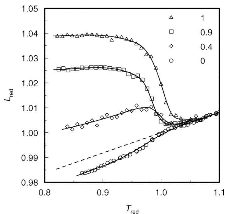
Figure 4 Dependence of the reduced sample lengths L_{\text{red}} (measured perpendicular to the helical axis) on the reduced temperature T_{\text{red}} = T/T_{\text{ci}} for several elastomers with different relative molar fractions x_{\text{odd}} of the nematic side group compound 3 . The dashed line indicates the expected dependence for an isotropic conformation obtained by extrapolation from a fit to the data of the isotropic phase.
