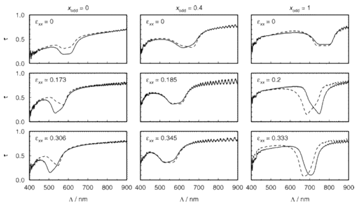
Figure 9 Transmission spectra of three elastomers with different relative molar fractions x_{\text{odd}} for light linearly polarized parallel (solid curves) and perpendicular (dashed curves) to the direction of stress at room temperature for different uniaxial strains \epsilon_{xx} .
