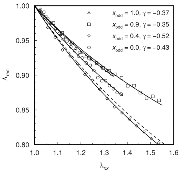
Figure 7 Dependence of the reduced center wavelength \Lambda_{\text{red}} of several elastomers with different relative molar fractions x_{\text{odd}} on the deformation \lambda_{xx} = 1 + \epsilon_{xx} . Solid lines: fits to the power law \lambda_{xx}^{\gamma} . Dashed line: expected power law for isotropic contraction ( \gamma = -1/2 ).
