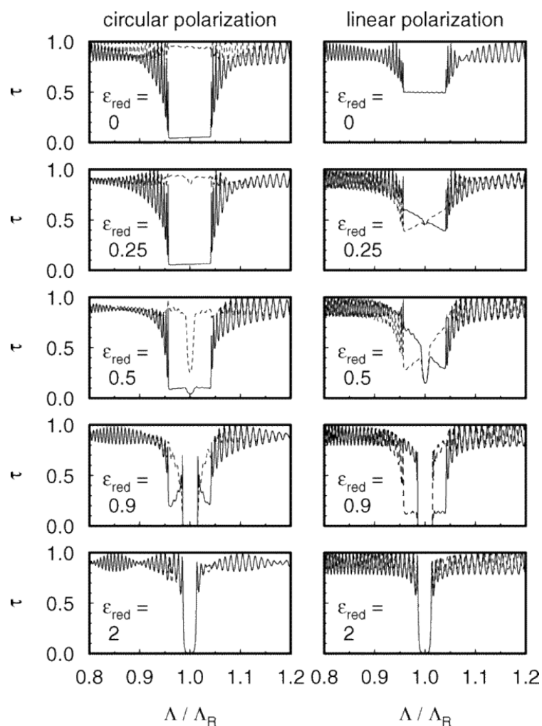
Figure 10 Transmission \tau of cholesteric elastomer films in dependence of the reduced wavelength \Lambda/\Lambda_R , calculated numerically according to theory 7,8 for a prolate conformation anisotropy r = 1.3 at different reduced strains \epsilon_{red} = \epsilon_{xx}/\epsilon_c . Left: transmission of left (solid curves) and right (dashed curves) circularly polarized light. Right: transmission of light linearly polarized parallel (solid curves) and perpendicular (dashed curves) to the direction of stress; for an oblate conformation with r = 1/1.3 the two linearly polarized spectra would have to be interchanged for each reduced strain.
