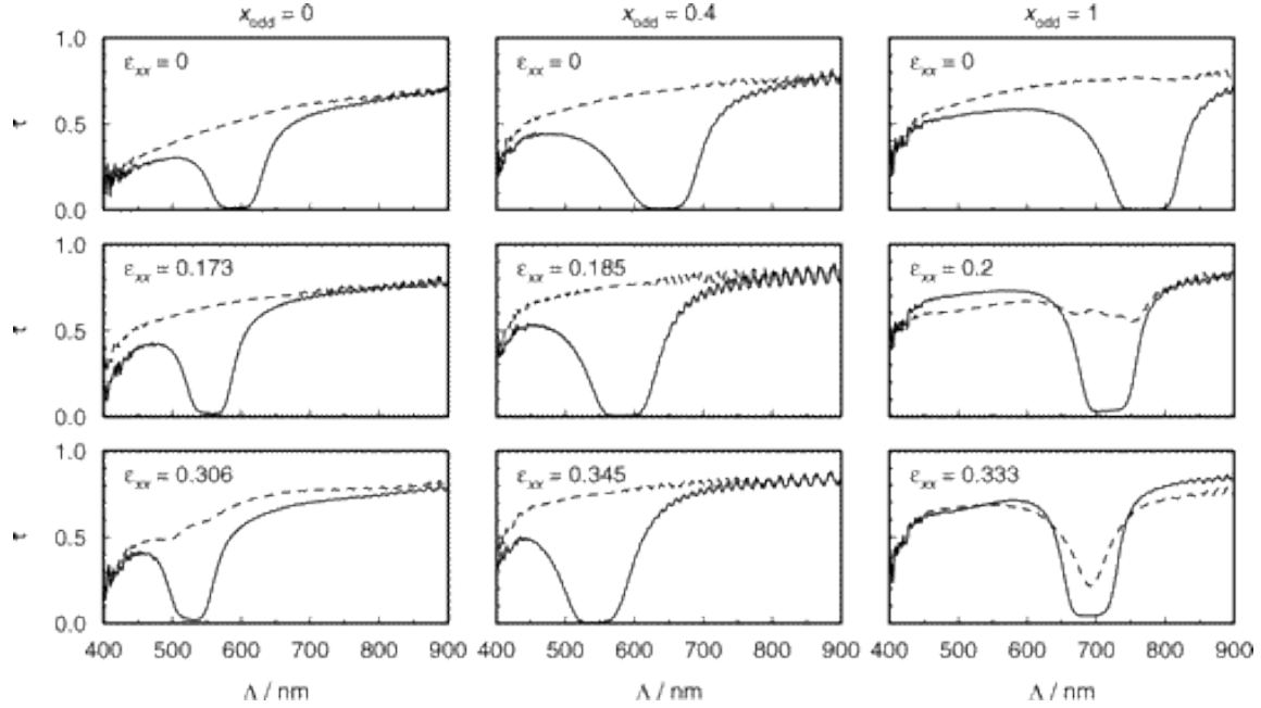
Figure 5 Transmission spectra of three elastomers with different relative molar fractions x_{\text{odd}} for left (solid curves) and right circularly polarized light (dashed curves) at room temperature for different uniaxial strains \epsilon_{xx} perpendicular to the helical axis.
