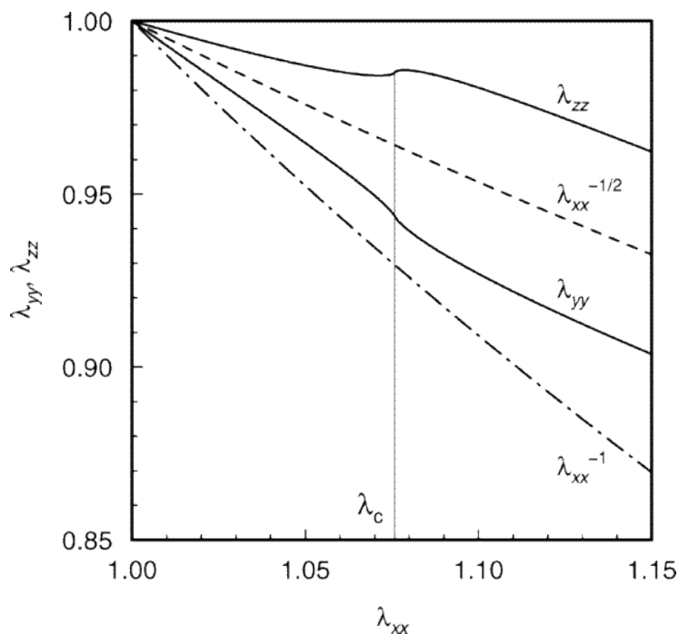
Figure 1 Deformations \lambda_{yy} and \lambda_{zz} of elastomer films, calculated numerically according to theory 7,8 in dependence of the deformation \lambda_{xx} for conformation anisotropies r = 1.3 or r = 1/1.3 (see text). Included are the power laws \lambda_{xx}^{-1/2} for an isotropic contraction and \lambda_{xx}^{-1} for a contraction along only one dimension. The critical deformation \lambda_c = 1 + \epsilon_c is indicated by the vertical line.
