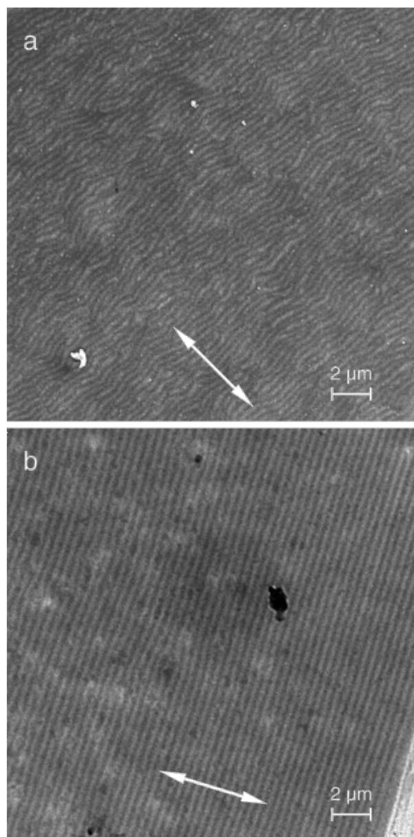
Figure 3 TEM micrographs of cholesteric elastomer films obtained by the anisotropic deswelling method (a) and by photo-cross-linking a well-aligned cholesteric polymer film (b). Cross sections along a direction perpendicular to the film surfaces are shown. Lines of equal brightness correspond to quasi-nematic planes with uniform orientation of the director in relation to the plane of observation. The average orientation of the cholesteric helix axes is indicated by double arrows.
