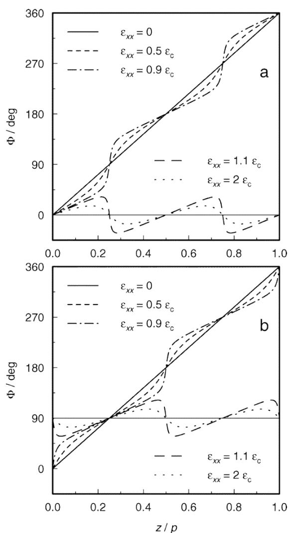
Figure 2 Director orientation angle \Phi(z/p) of elastomer films, calculated numerically according to theory 7,8 for different strains \varepsilon_{xx} in units of the critical strain \varepsilon_c = 0.0758 (a) for a prolate conformation anisotropy r = 1.3 and (b) for an oblate conformation anisotropy r = 1/1.3 (see text).
