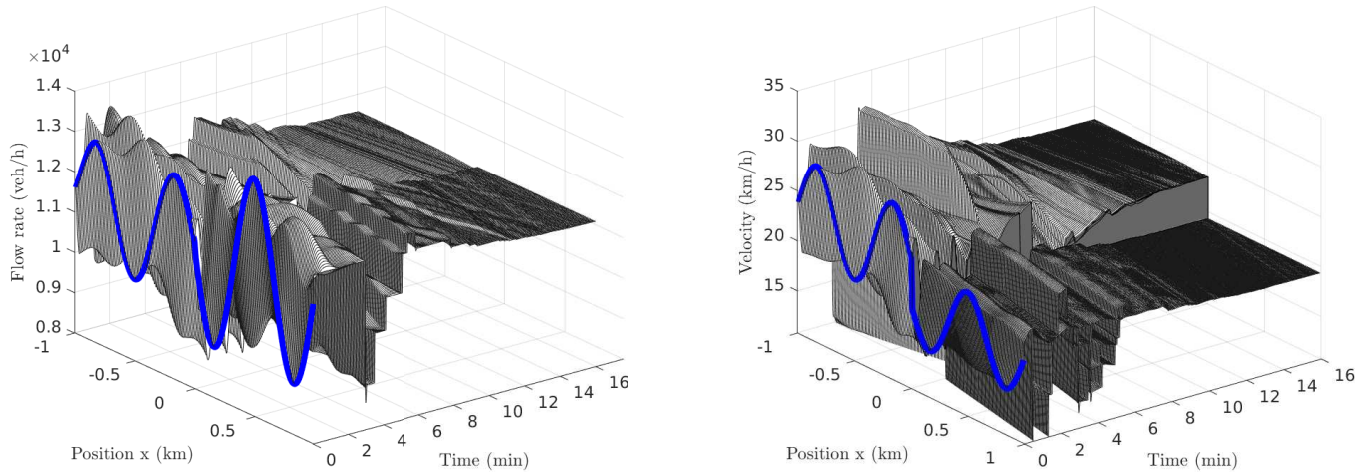
FIGURE 5 Numerical solution of the flow rate and velocity with the ramp metering event-triggered boundary control U_{\text{nom}}(t_k) (96)-(98).
