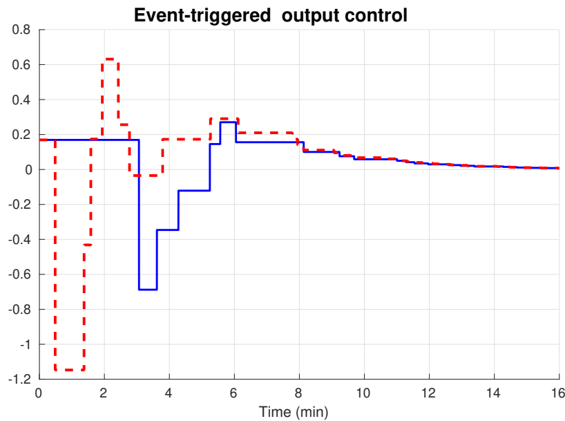
FIGURE 6 Time-evolution of the event-triggered boundary output control. The updating is aperiodically, according to the dynamic triggering condition (96), under the cases i) \theta_2 = 1.98 (blue line) and ii) \theta_2 = 10^9 (red dashed-line) which corresponds to the limiting case in which one deals with a “static triggering condition” as discussed in Remark 3.
