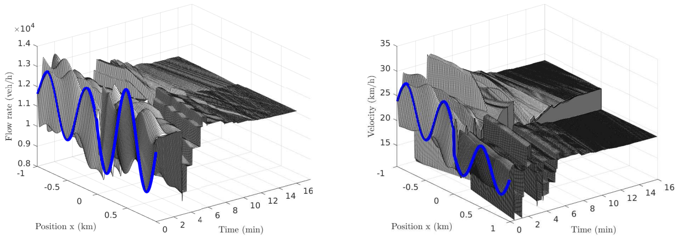
FIGURE 5 Numerical solution of the flow rate and velocity with the ramp metering event-triggered boundary control U_{nom}(t_k) (96)-(98).
