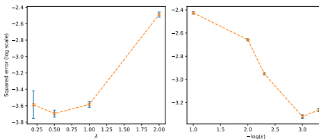
Figure 7: 6D experiment: On the left, \|\hat{z}_\lambda - z_0\|_{L^2(\bar{\mu})}^2 (our model) and on the right, \|\hat{z}_\varepsilon - z_0\|_{L^2(\bar{\mu})}^2 (Sinkhorn).
