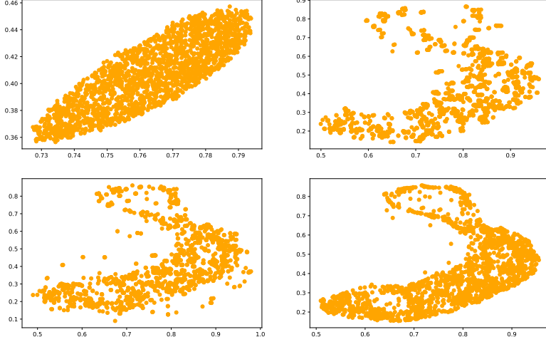
Figure 6: Pushforwards \nabla \hat{f}(\hat{\mu}_{test}) . From top left to bottom right: Sinkhorn ( \varepsilon = 0.1 ), SSNB ( \lambda = 0.2, M = +\infty ), Semi-dual OT ( \lambda = 0.2, L = 1 ), Sinkhorn ( \varepsilon = 0.0001 ).
