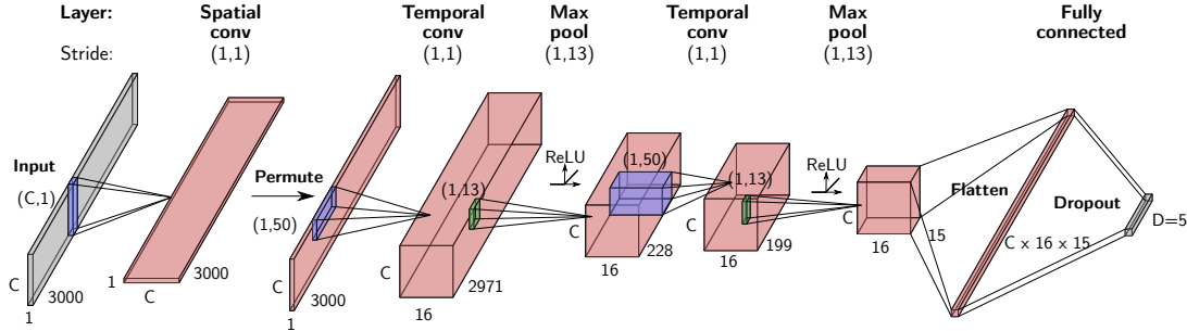
Figure 8: Neural network architectures f_{\Theta} used in (1) pathology detection and (2) sleep staging experiments.
