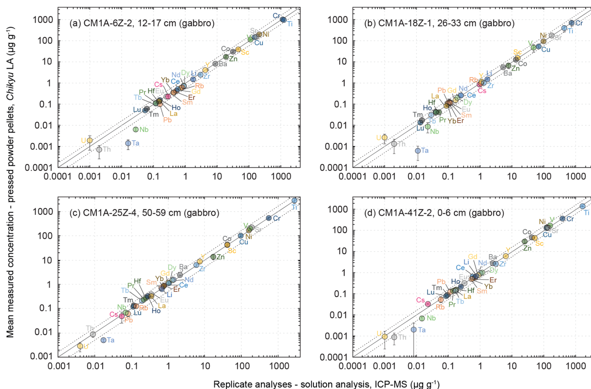
Figure 6. Comparison of the mean measured concentrations obtained by LA-ICP-MS on pressed powder pellets with the analysed replicates for the same samples (solution analysis, University of Southampton, UK) for four gabbro samples from Hole CM1A. The selected samples are (a) CM1A-6Z-2, 12–17 cm ( n = 5 ), (b) CM1A-18Z-1, 26–33 cm ( n = 5 ), (c) CM1A-25Z-4, 50–59 cm ( n = 6 ), and (d) CM1A-41Z-2, 0–6 cm ( n = 6 ). The black solid line is the 1 : 1 line between the concentrations determined by LA-ICP-MS on-board the D/V Chikyu and for the replicates. The black dashed lines represent 50 % deviation from the 1 : 1 line.
