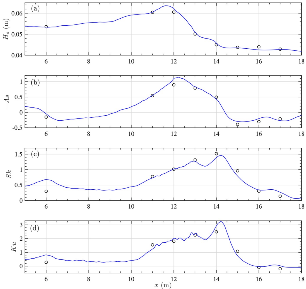
Figure 12: Spatial evolution of wave statistics computed from the experiments (circles) and simulations with Mis-b005 (solid line) for the irregular wave case of Beji and Battjes (1993) (JONSWAP spectrum with H_s = 0.049 m and T_p = 2.5 s). Waves break over the bar in the model and in the experiments (plunging breakers).
