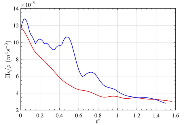
Figure 4: Comparison of the instantaneous energy dissipation rate \Pi_b(t) calculated for the plunging BB-regular case in the Misthyc model using: (blue) the HJ analogy Eq. (13), or (red) the Mis-b005 Eq. (15) parameterization with b = 0.05 .
