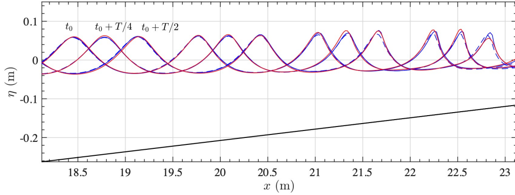
Figure 5: Sensitivity of the simulation results to the spatial discretization for the HS test case using the NWT (blue dashed, L/\Delta x = 35 , and blue solid, L/\Delta x = 50 ) and Misthyc (solid red with L/\Delta x = 70 ) model.
