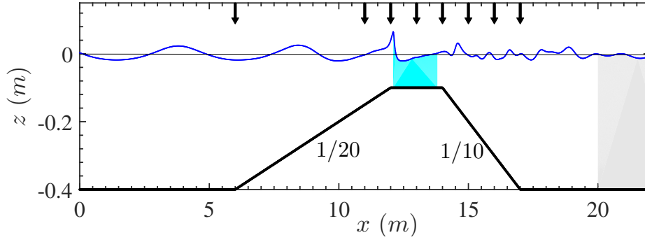
Figure 9: Set-up of the computational domains in the simulations of the Beji and Battjes (1993) experiments for periodic waves shoaling and plunging breaking over a bar (BB). Arrows indicate the locations of wave gauges in the experiments and simulations. Wave breaking occurs in the models in the cyan shaded region, from onset to termination, and the gray shaded region indicates the absorbing beach. Note, the free surface shown is of BB-regular.
