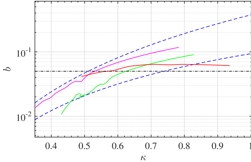
Figure 15: Evolution of the instantaneous breaking strength b calculated with the HJ model during breaking simulations with Misthyc for the (Table 3): (a) HS (solid magenta), (b) TK (solid green), and (i) BB-regular (solid red) periodic spilling/plunging breaking wave experiments, as a function of \kappa = H/d . The dashed blue curves represent the lower ( b_{min} ) and upper ( b_{max} ) bounds estimated for b , and the horizontal dash-dotted black line is b = 0.05 .
