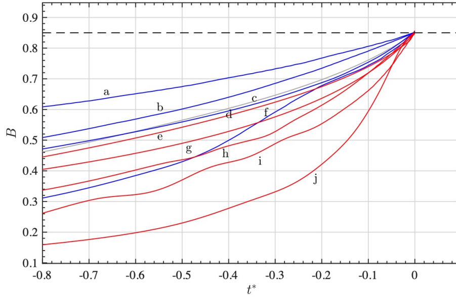
Figure 16: Evolution of B = u/c as a function of non-dimensional time t^* = (t - t_b)/T_b , referred to the time of breaking onset, up to breaking onset ( B = 0.85 ; horizontal dashed line), computed for a wave crest evolving over sloping bathymetries in the experimental test cases listed in Table 3. Red lines for P-cases and blue lines for S-cases have smaller and larger values of dB/dt at breaking onset, respectively.
