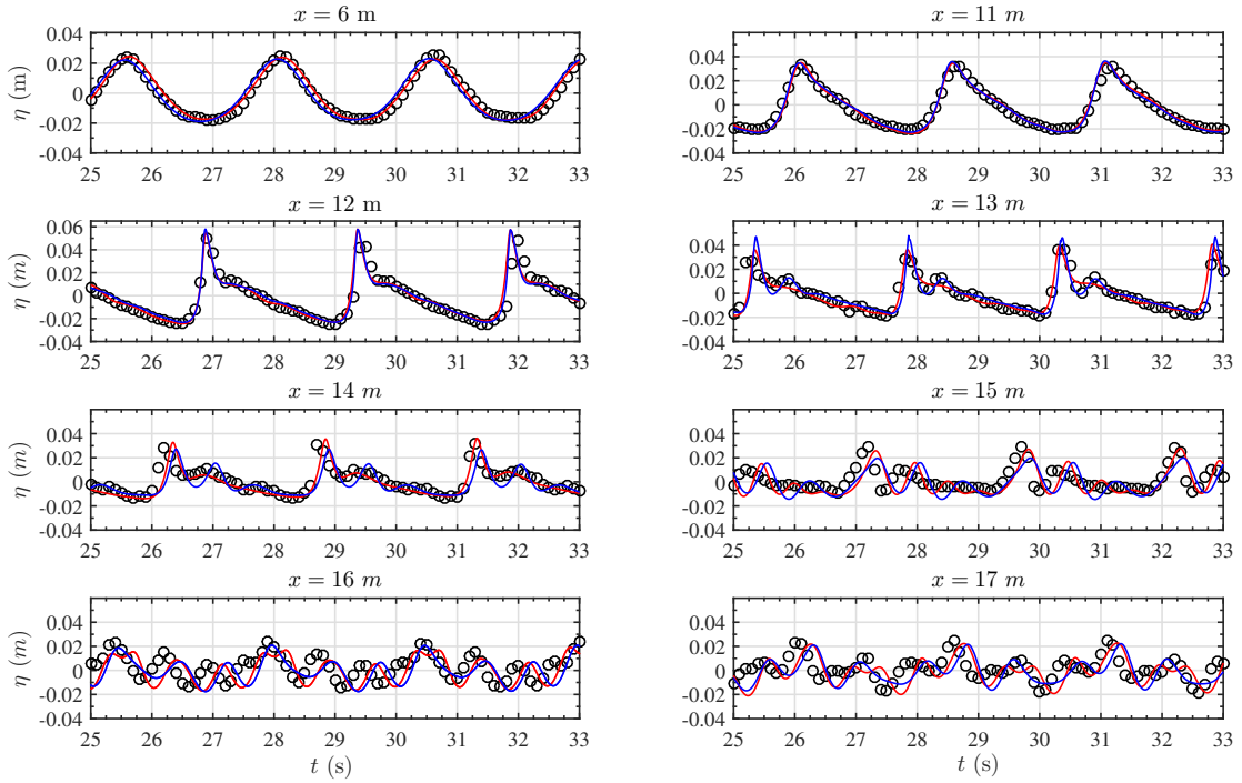
Figure 10: Comparison of the temporal evolution of the free surface at the gauge locations from the Beji and Battjes (1993) test case for regular plunging waves (circles) with Mis-b005 (red solid line) and NWT-b005 (blue solid line).
