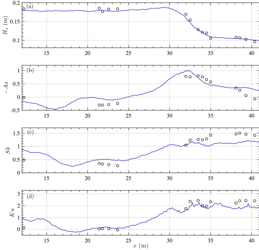
Figure 14: Spatial evolution of wave statistics computed based on results of experiments (circles) and simulations with Mis-b005 (solid line) for the irregular wave case of Adytia et al. (2018) ( H_s = 0.2 m and T_p = 2.5 s); waves break over the bar in the model and in the experiments.
