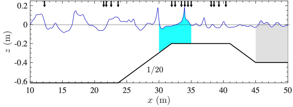
Figure 13: Set-up for simulations with Misthyc of Adytia et al. (2018) experiments for irregular waves propagating over a bar ( H_s = 0.2 m and T_p = 2.5 s), with arrows showing the location of the 15 wave gauges. The cyan shading shows the breaking region from onset to termination, and the gray shading indicates the absorbing beach region.
