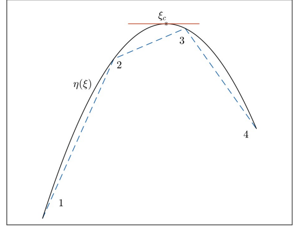
Figure 17: Sketch showing the calculation of a local wave crest location between discretization points on the simulated free surface.
