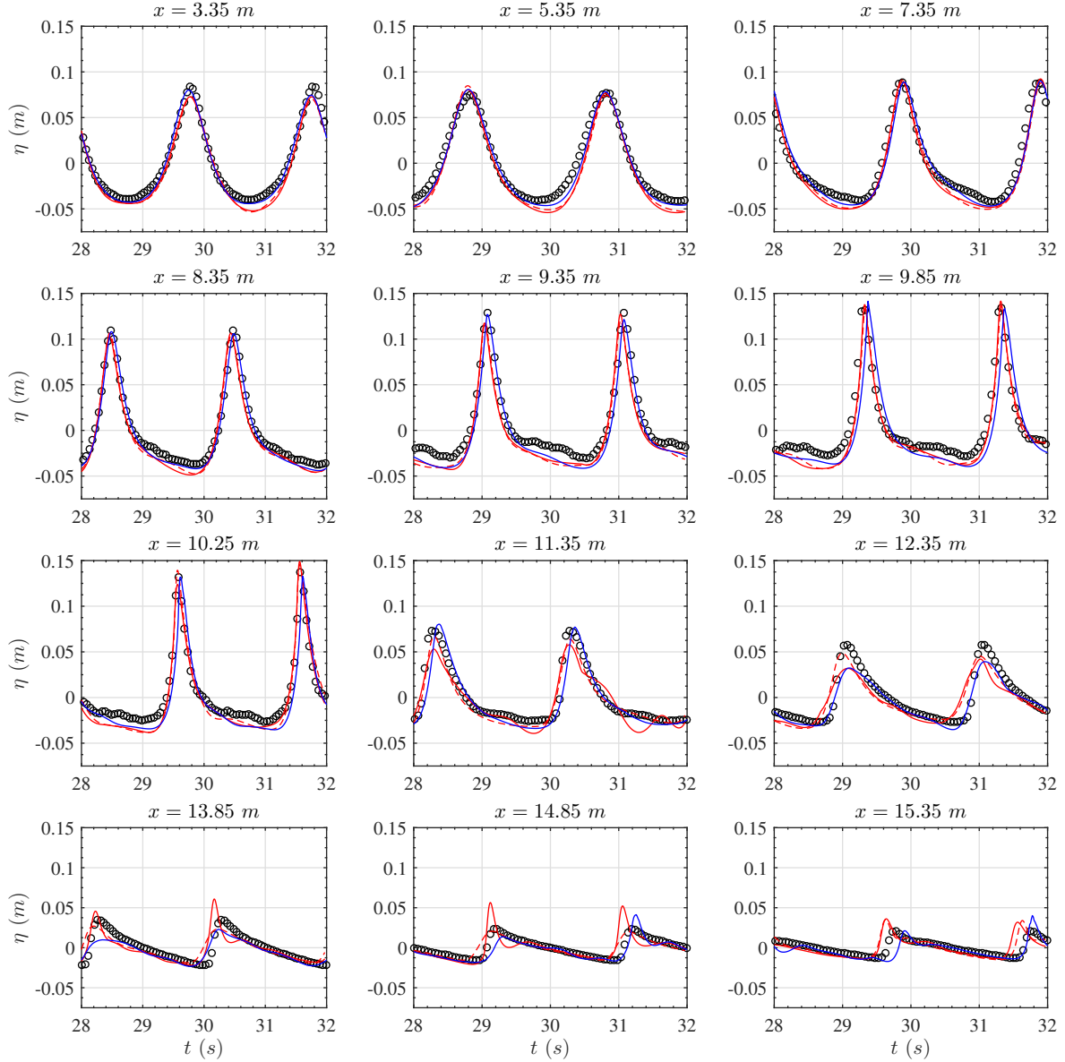
Figure 8: Comparison of the temporal evolution of the free surface position measured at the gauge locations from Ting and Kirby (1994) for regular spilling waves (circles) with simulations using Misthyc with the HJ model (dashed red line), Mis-b005 (solid red line), and NWT-b005 (solid blue line).
