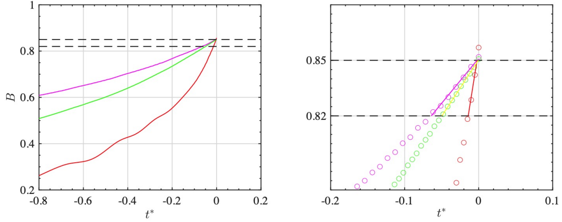
Figure 2: Evolution of B = u/c in simulations with the Misthyc model as a function of non-dimensional time t^* = (t - t_b)/T_b ( t_b denotes the time of breaking onset when B = B_{th} = 0.85 ), for periodic: (i) plunging breaking waves propagating over a bar, from Beji and Battjes (1993) (BB-regular, red); (ii) spilling breaking waves propagating over a plane slope, from Hansen and Svendsen (1979) (HS, magenta); and shoaling and spilling breaking waves propagating over a plane slope, from Ting and Kirby (1994) (TK, green).
