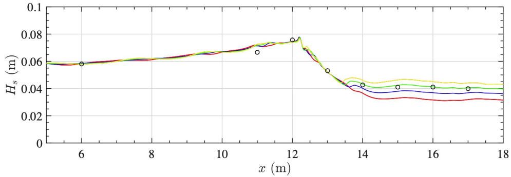
Figure 11: Spatial evolution of the significant wave height H_s for the BB-regular experiments (circles) and simulations with the Mis-b005 model using different breaking termination criteria B_{\text{off}} = : (red) 0.2, (blue) 0.25, (green) 0.30, and (yellow) 0.35.
