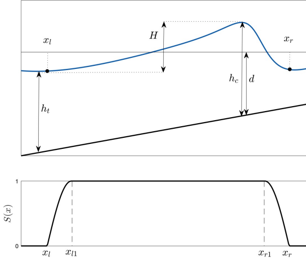
Figure 1: (top) Geometric parameters used to calculate the HJ dissipation, and (bottom) the shape function S(x)
