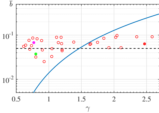
Figure 3: Average breaking strength \bar{b} computed for the HJ parameterization, as a function of \gamma for depth-limited breaking waves simulated in Misthyc including: (filled circles) regular wave cases, magenta: HS, green: TK and red: BB; (hollow circles) BB-irregular cases. For comparison, the empirical parameterization from Eq. 16 proposed by Derakhti et al. (2018a), is indicated with a solid line. The dashed line shows the constant strength average breaking value b = 0.05 used in the Mis-005 parameterization.
