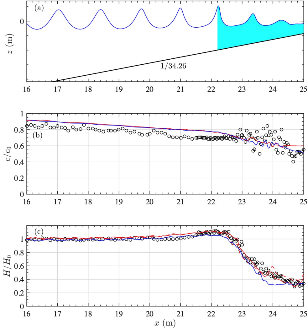
Figure 6: (a) Bathymetry of the Hansen and Svendsen (1979) (HS) experimental set-up for periodic shoaling and spilling breaking waves, where the shaded cyan region indicates the wave crest location from the onset of wave breaking (note an absorbing beach is specified in the models for x \geq 25.5 m). Spatial evolution of the (b) wave celerity, and (c) wave height in the experimental data (circles), Misthyc using the HJ model (dashed red line), Mis-b005 (solid red line) and NWT-b005 (solid blue line), averaged over 5 successive wave periods after a quasi-steady state is reached.
