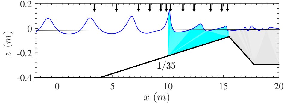
Figure 7: Setup for Ting and Kirby (1994) laboratory experiments of periodic spilling breakers propagating over a 1/35 slope, with black arrows showing the locations of the 12 wave gauges. The cyan shading indicates the simulated wave breaking region, from onset to termination. The gray shading indicates the beach absorption zone.
