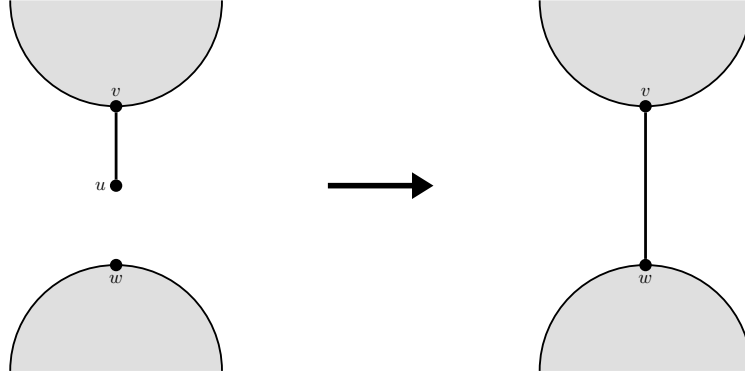
(b) Attaching u at w
