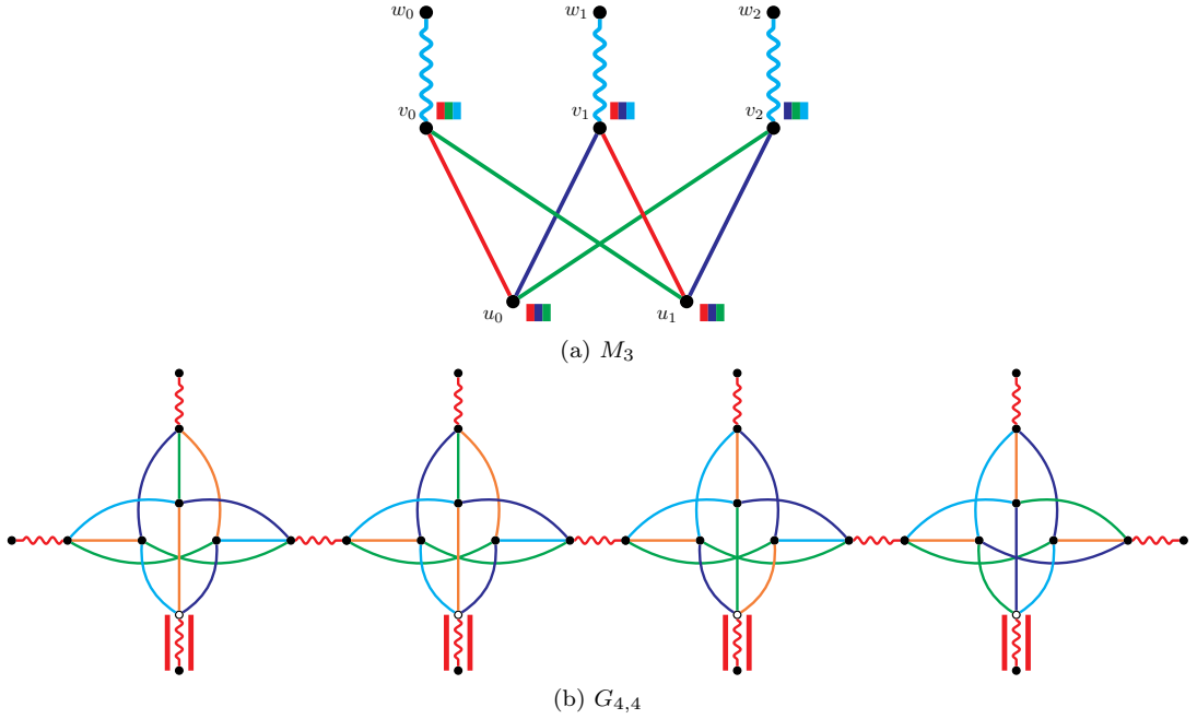
Figure 1: The gadgets M_3 and G_{4,4} from Section 2. In (a), wiggly edges are outputs. In (b), wiggly edges are outputs of the four copies of M_4 in G_{4,4} , those surrounded by bold lines being the four outputs of G_{4,4} . In (b), the white vertices are the four support vertices of G_{4,4} . In each case, is also given an AVD edge-colouring using the least number of colours possible (4 in (a), 5 in (b)). In (a), the set of incident colours is given for every vertex of maximum degree (3). Note also that, in (b), the edges of the four copies of M_4 are not coloured the same way, to illustrate the fact that, in an AVD 5-edge-colouring of G_{4,4} , even though we have some control over the sets of incident colours achieved for the support vertices, we have less control on how those sets are obtained.
