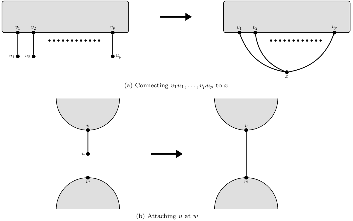
Figure 2: Illustration of the connection and attachment operations.
