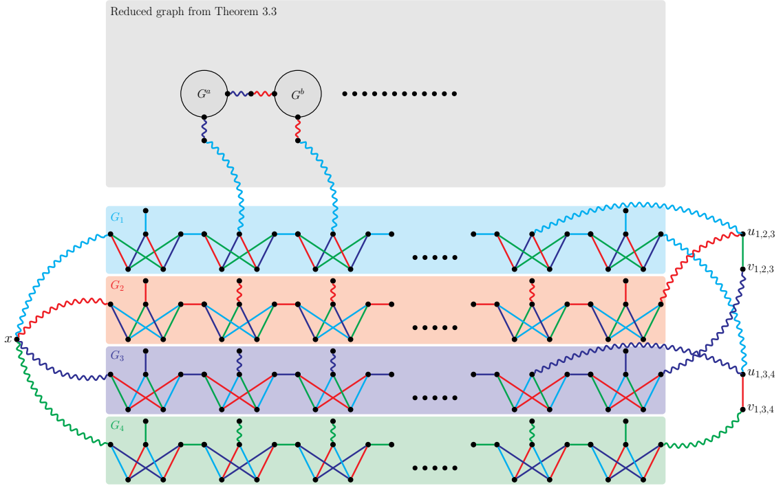
Figure 4: Part of the reduction in the proof of Theorem 4.3, in the special case where k = 4 . Wiggly edges are outputs of some G_{k,r} . Due to space limitation, note that not all pairs \{u_{i,j,\ell}, v_{i,j,\ell}\} are represented.
