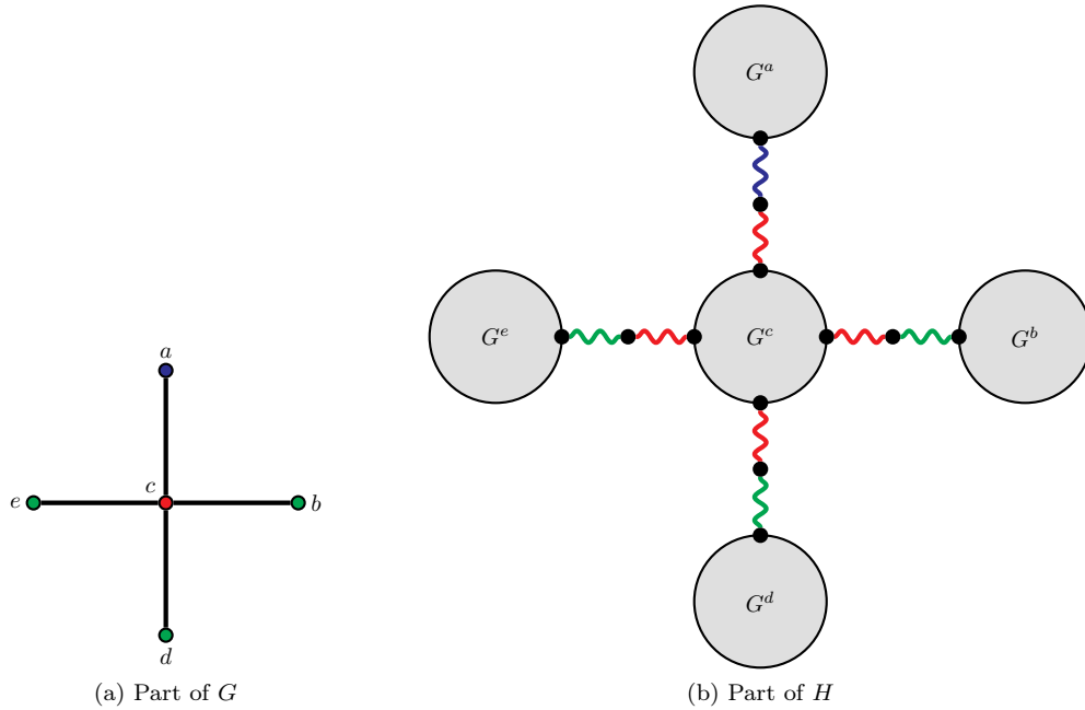
Figure 3: Illustration of the reduction in the proof of Theorem 3.3. (a) depicts part of a graph G and of a proper vertex-colouring. (b) depicts part of the reduced graph H and of a corresponding AVD edge-colouring. In (b), wiggly edges of H are outputs of the G^v 's.
