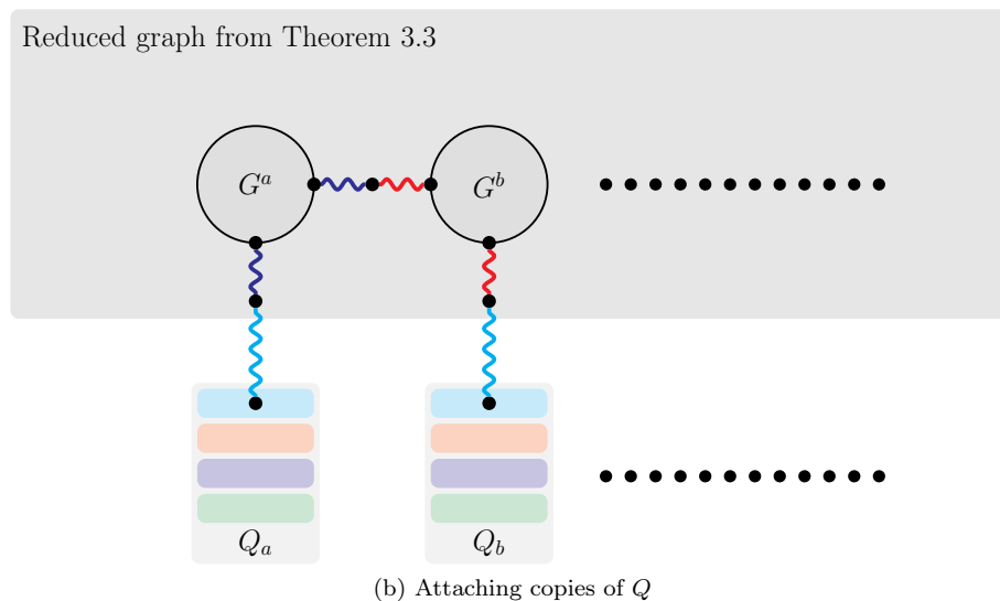
Figure 5: Part of the reduction in the proof of Theorem 4.5, in the special case where k = 4 . Wiggly edges are outputs of some G_{k,r} . Due to space limitation, note that, in (a), not all pairs \{u_{i,j}, v_{i,j}\} are represented.
