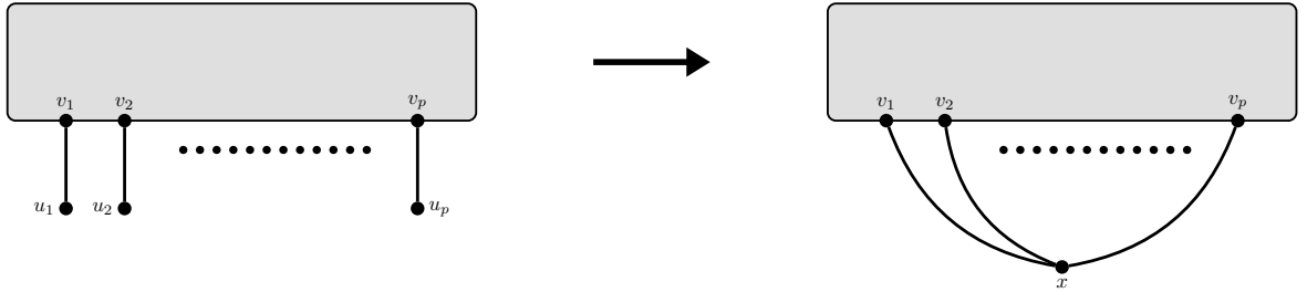
(a) Connecting v_1u_1, \dots, v_pu_p to x
