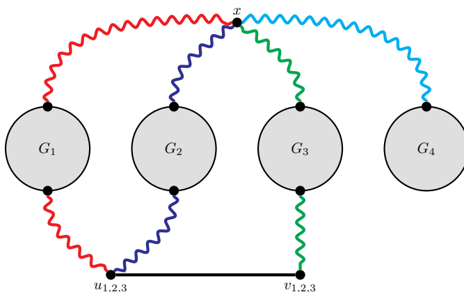
Figure 3: (Part of) how the G_i 's connect in the proof of Theorem 4.3. Wiggly edges of H are outputs of the G_i 's.
