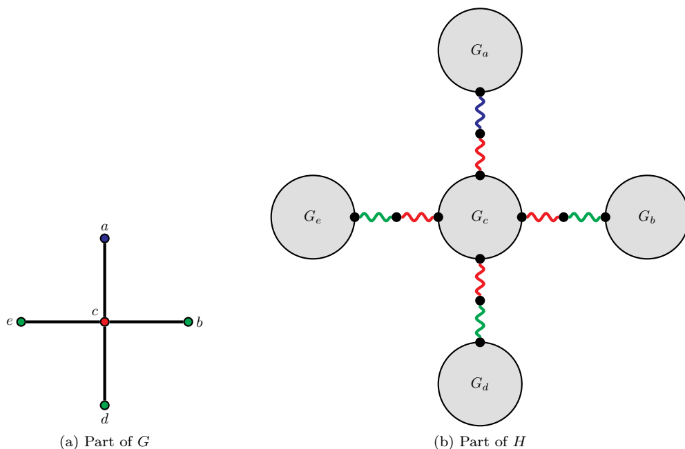
Figure 2: Illustration of the reduction in the proof of Theorem 3.3. (a) depicts part of a graph G and of a proper vertex-colouring. (b) depicts part of the reduced graph H and of a corresponding avd edge-colouring. Wiggly edges of H are outputs of the G_v 's.
