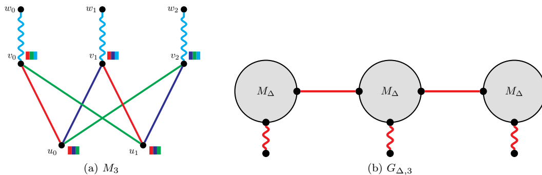
Figure 1: The gadgets M_3 and G_{\Delta,3} from Section 2. In each case, the coloured edges are part of an avd edge-colouring using the least number of colours possible (4 in (a), \Delta + 1 in (b)). In (a), the set of incident colours is given for every vertex of maximum degree (3). Wiggly edges are outputs.
