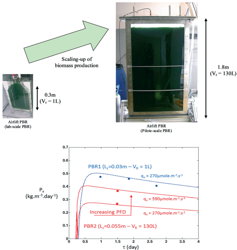
Fig. 14 Comparison of the volumic productivity in PBR of different sizes and comparison the model of eqn (27)–(29) with for Neochloris oleoabundans : \rho_M = 0.8 , \varphi_M = 1.83 \times 10^{-9} kg per \mu\text{mole} , K = 90 \mu\text{mole per m}^2 \text{s}^{-1} .
