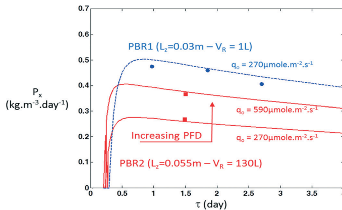
Fig. 14 Comparison of the volumic productivity in PBR of different sizes and comparison the model of eqn (27)–(29) with for Neochloris oleoabundans : \rho_M = 0.8 , \phi_M = 1.83 \times 10^{-9} \text{ kg per } \mu\text{mole} , K = 90 \mu\text{mole per } \text{m}^2 \text{ s}^{-1} .
