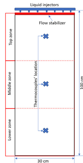
Fig. 1 – (a) Schematic description of indoor Algofilm ©. (b) Experimental setup for Algofilm © indoor prototype. (c) Flow for uniform film distribution and (d) Distribution of the thermocouples on sub-system “Flowing liquid”.
