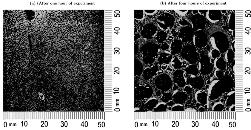
Fig. 5 – Development of irregular condensate film on T_1 = 50\text{ °C} and \phi = 6^\circ .
