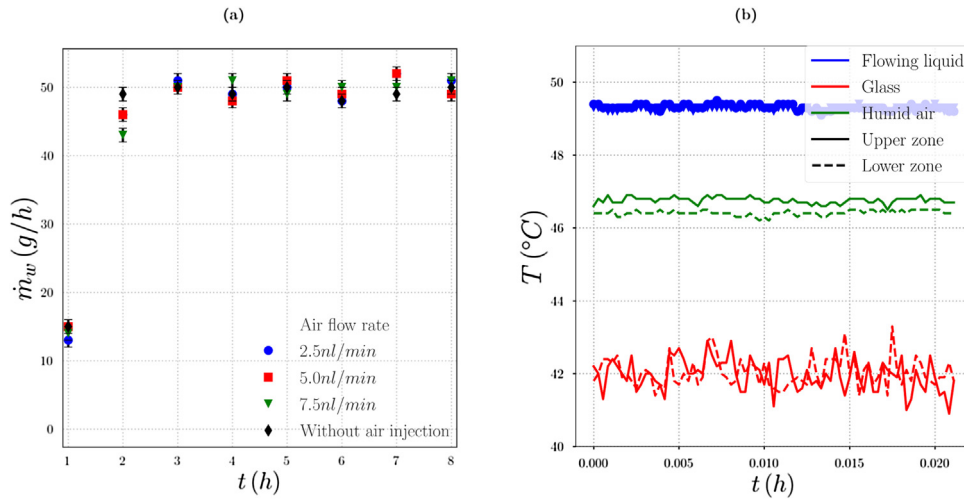
Fig. 7 – Experimental validation of theoretical assumptions: (a) Effect of air injection on condensation rate; (b) Temperature gradient of each subsystem for T_l = 50\text{ }^\circ\text{C} (without air injection).
