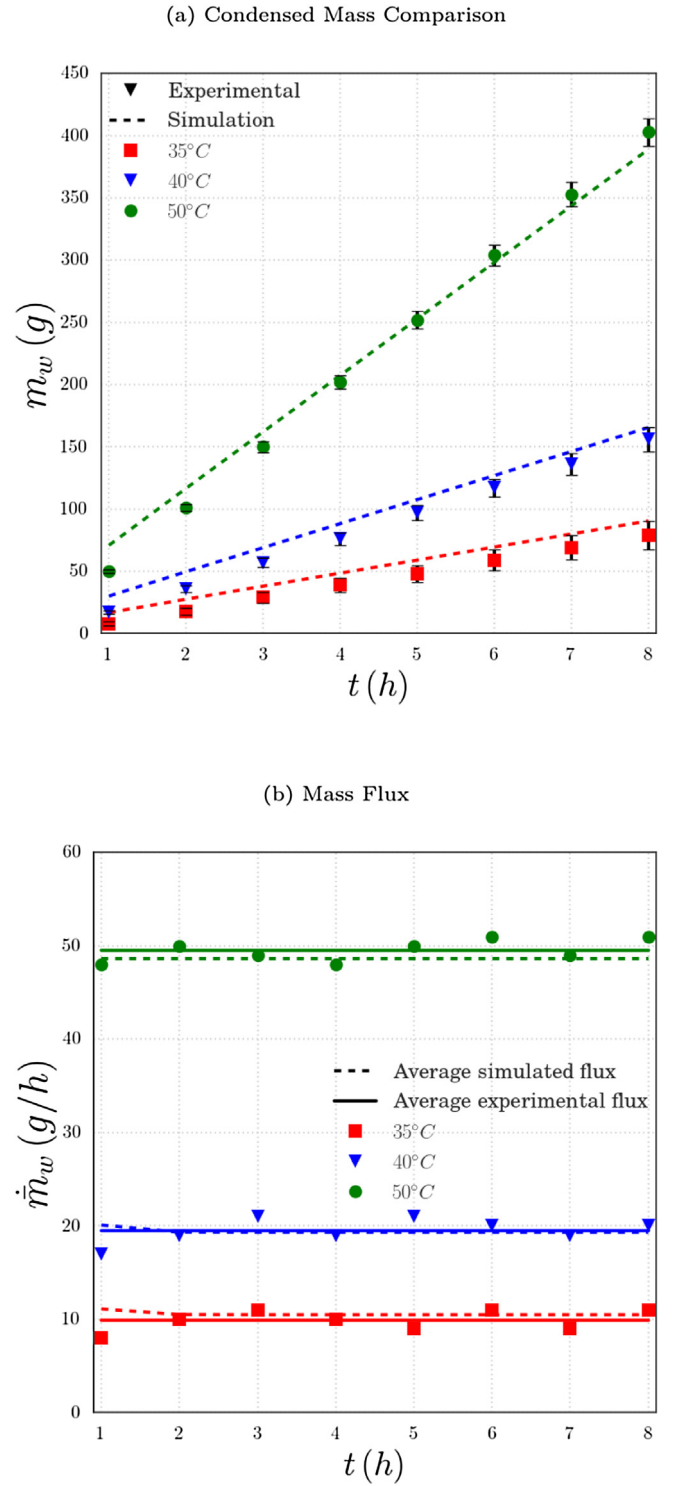
Fig. 10 – Comparison of experimental and simulated results for T_l = 35, 40, 50 °C: (a) Condensed mass (b) Mass flux.
