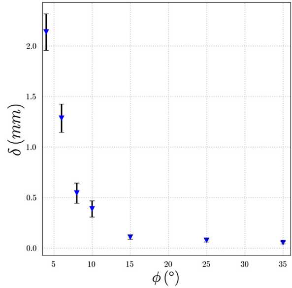
Fig. 6 – Estimation of averaged condensate film thickness over the range of inclination angles \phi .
