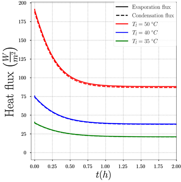
Fig. 9 – Evolution of evaporation and condensation latent heat fluxes for T_l = 35, 40, 50 °C.
