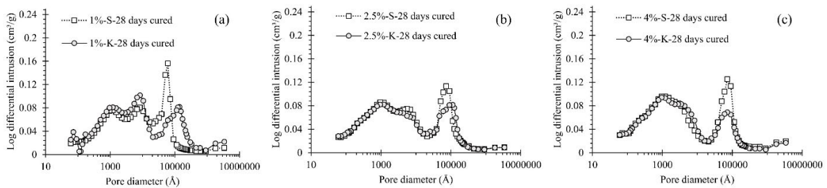
270 Fig. 3 Comparative evolution of PSD in the 1% (a), 2.5% (b), and 4% (c) lime-treated statically and Kneading compacted 28- 271 days cured specimens 272
