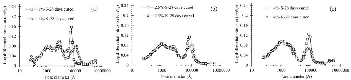
270 271 Fig. 3 Comparative evolution of PSD in the 1% (a), 2.5% (b), and 4% (c) lime-treated statically and Kneading compacted 28- 272 days cured specimens
