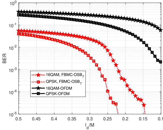
Fig. 4. Timing offset evaluation in terms of BER for the OSB 7 -FBMC and OFDM receivers over the 5G QuaDRiGa fading channel under the '3GPP-3D-UMA-NLOS' scenario', with 4 users and 64 Rx antennas.
