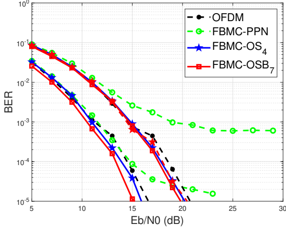
Fig. 2. BER performance comparison of different receivers over the 5G QuaDRiGa fading channel under the '3GPP-3D-UMA-NLOS' scenario', with 4 users and 64 Rx antennas.
