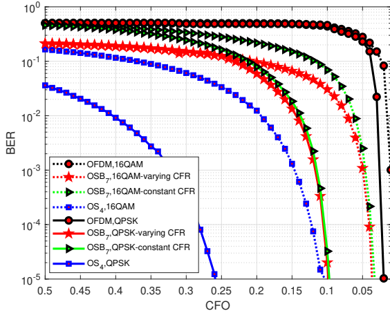
Fig. 6. Carrier frequency offset evaluation in terms of BER for different receivers with 4 users and 64 Rx antennas.
