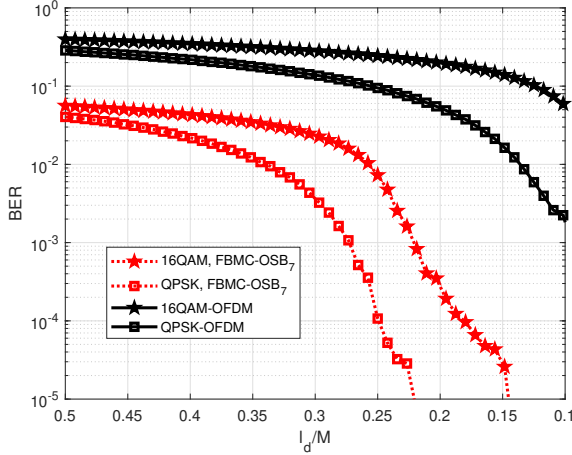
Fig. 4. Timing offset evaluation in terms of BER for the OSB 7 -FBMC and OFDM receivers over the 5G QuaDRiGa fading channel under the '3GPP-3D-UMA-NLOS' scenario', with 4 users and 64 Rx antennas.
