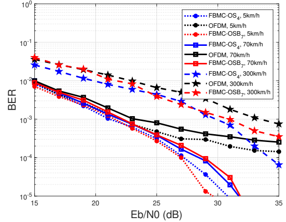
Fig. 5. BER performance for different receivers over the non-static 5G QuaDRiGa fading channel under the '3GPP-3D-UMA-NLOS' scenario', with 4 users and 64 Rx antennas.
