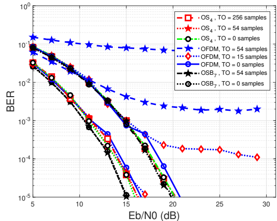
Fig. 3. BER performance comparison of different receivers in the presence of timing offset over the 5G QuaDRiGa fading channel under the '3GPP-3D-UMA-NLOS' scenario', with 4 users and 64 Rx antennas.
