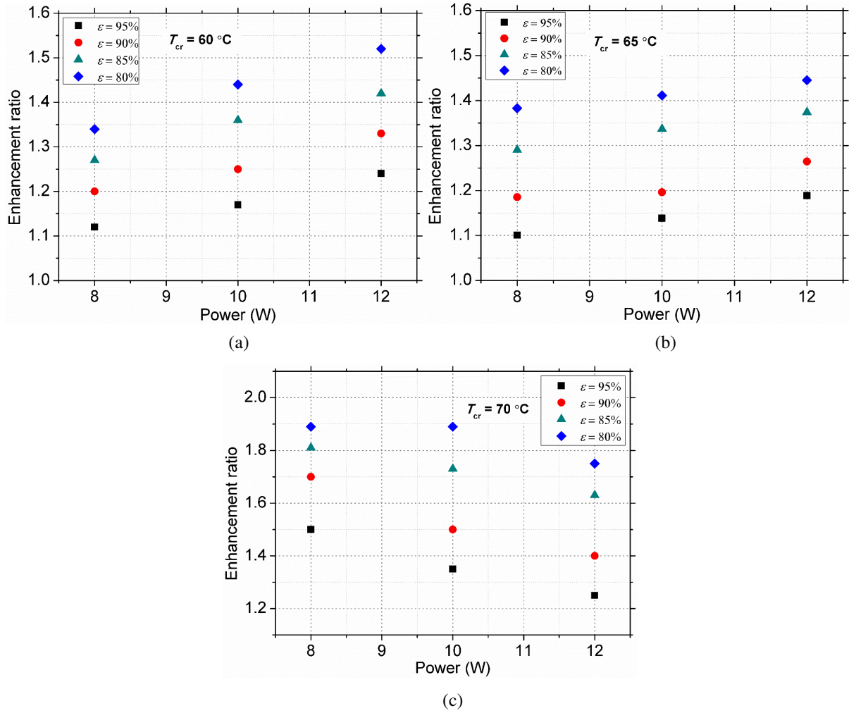
Fig. 9. Enhancement ratio of heat sinks using SPMs of various porosities for three critical temperatures of (a) 60 °C, (b) 65 °C, and (c) 70 °C.
