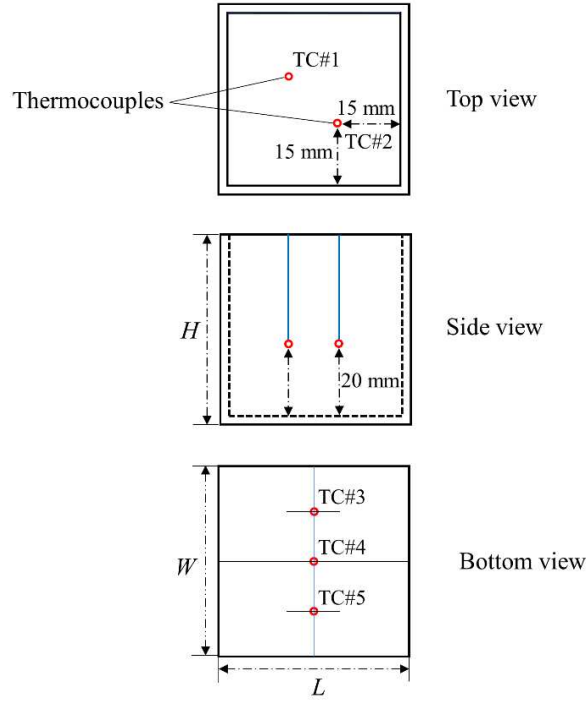
Fig. 4. Thermocouple distribution positions.
