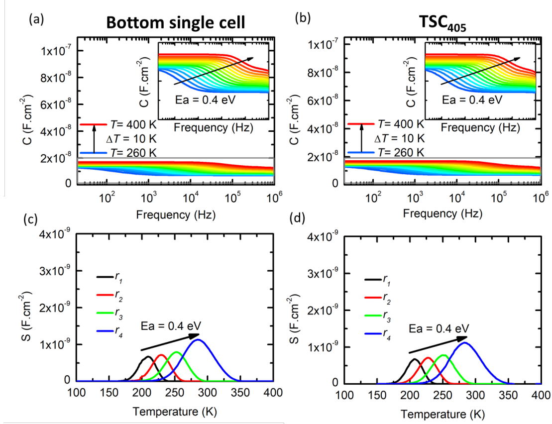
Fig. 8. (a) AS results of the Bottom subcell modelled alone at 0 V DC; (b) AS results of the TSC 405 under a light power density of 1 W.cm -2 and polarized at the open-circuit value of the absorbing Top subcell; (c) DLTS results of the Bottom subcell modelled alone; (d) DLTS results of the TSC 405 under a light power density of 1 W.cm -2 .
