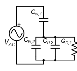
Fig. 4. Simplified AC circuit of the TSC if we consider the contribution of diffusion phenomena in the bottom subcell. C_{w,1} is the depletion-layer capacitance of the Top subcell, C_{w,2} , C_{D,2} and G_{D,2} are the depletion-layer capacitance, diffusion capacitance and diffusion conductance of the Bottom subcell, respectively.
