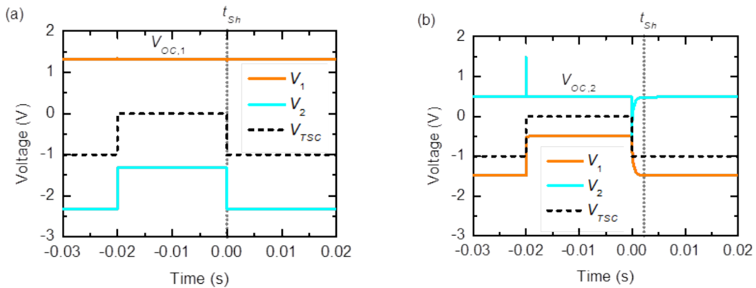
Fig. 7. Distribution of the applied voltage between the subcells versus time (a) in the TSC 405 case and (b) in the TSC 980 case at 300 K under 1 \text{ W.cm}^{-2} light bias.
