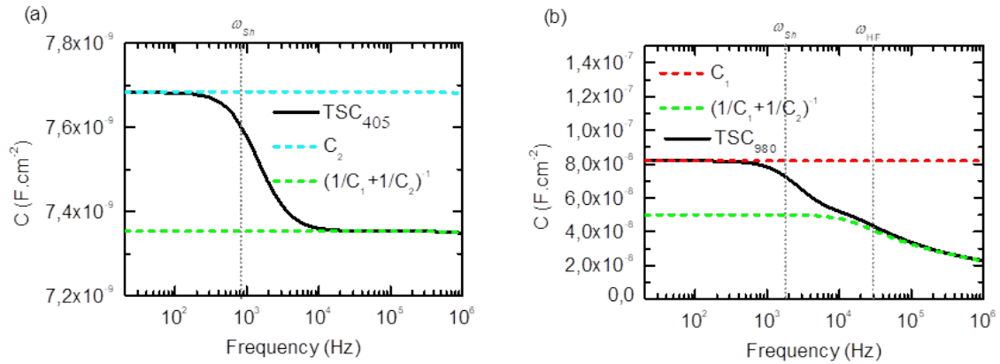
Fig. 6. C(f) curves modelled at 300 K from (a) the TSC, the Bottom subcell and (1/C_1 + 1/C_2)^{-1} in the TSC 405 case without defects under 1 \text{ mW.cm}^{-2} light bias and (b) the TSC, the Top subcell and (1/C_1 + 1/C_2)^{-1} in the TSC 980 case without defects under 1 \text{ mW.cm}^{-2} light bias.
