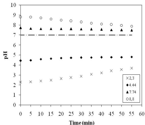
Fig. 8. Evolution of pH values during EC for different values of initial pH: C_0 = 50 \text{ mg L}^{-1} , j = 300 \text{ A m}^{-2} , Q = 15 \text{ L h}^{-1} , e = 1\text{cm} , \kappa = 2.5 \text{ mS cm}^{-1}
