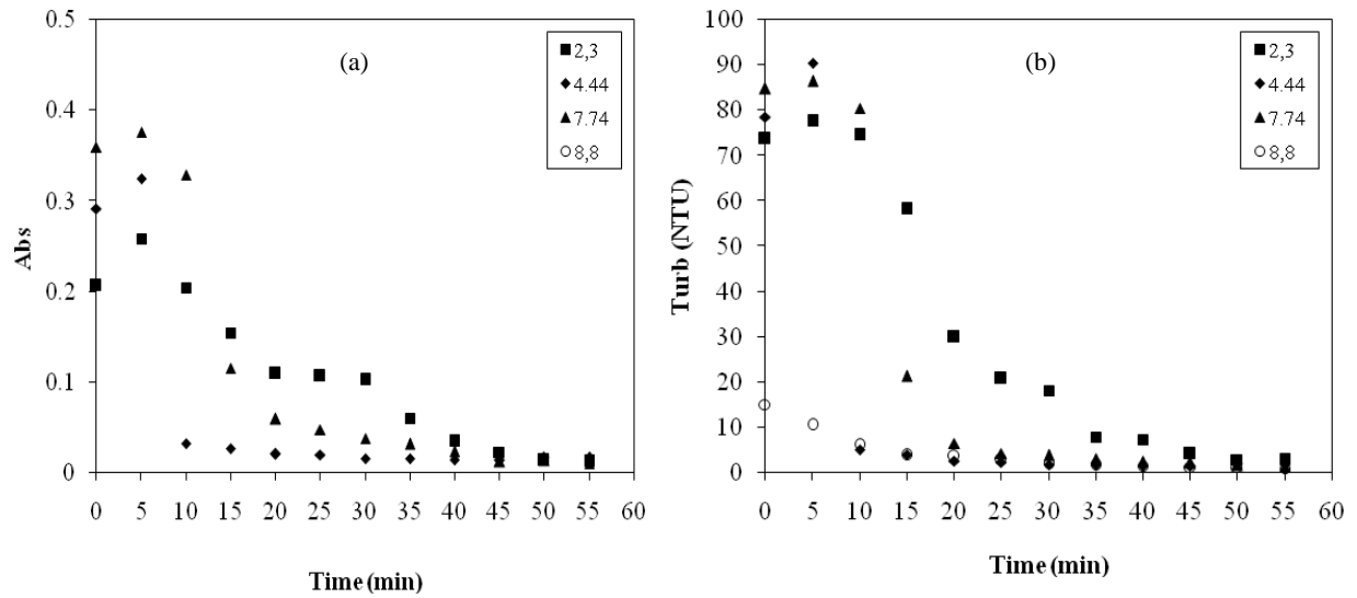
Fig. 7. Evolution of absorbance (a) and turbidity (b) during the treatment for different values of initial pH: C_0 = 50 \text{ mg L}^{-1} , j = 300 \text{ A m}^{-2} , Q = 15 \text{ L h}^{-1} , e = 1\text{cm} , \kappa = 2.5 \text{ mS cm}^{-1}
