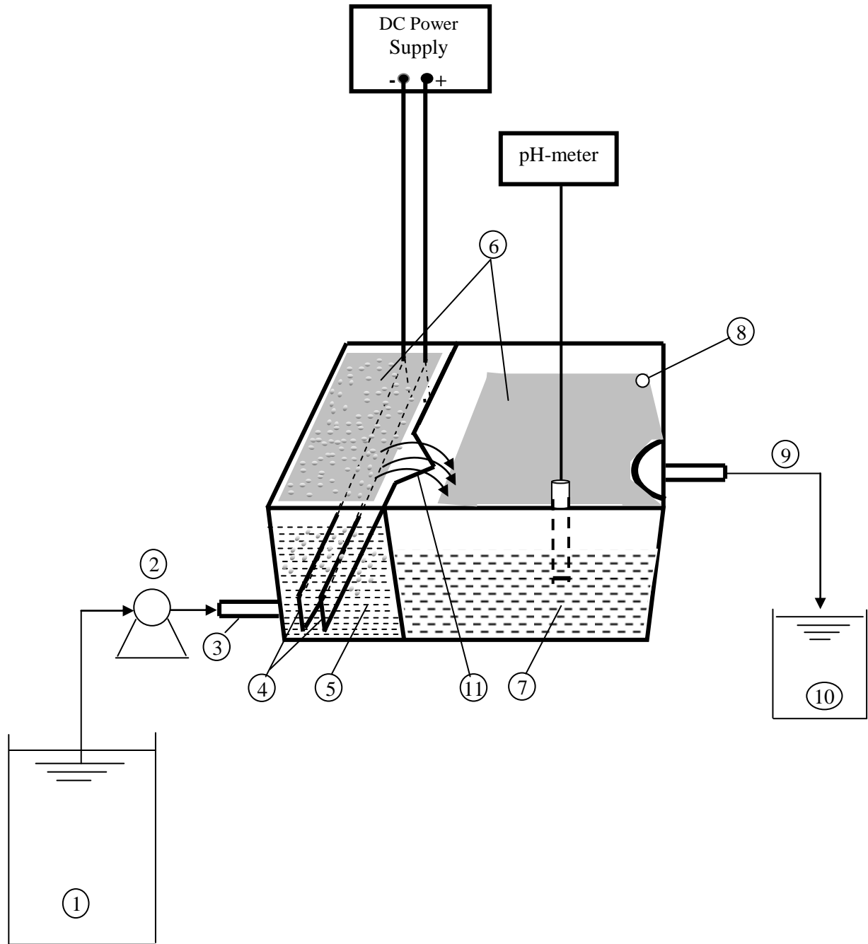
Fig.2. Experimental setup of continuous EC cell (1: wastewater tank; 2: peristaltic pump; 3: inlet of the first compartment; 4: electrodes; 5: first chamber; 6: sludge; 7: second chamber; 8: sludge exit (overflow); 9: treated effluent outlet; 10: treated water tank; 11: outfall).
