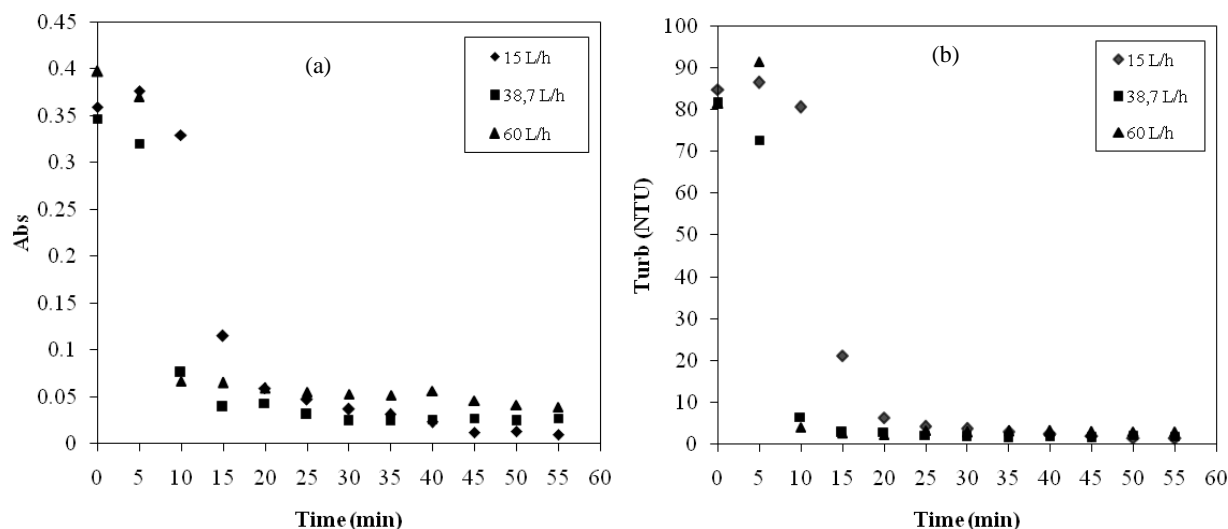
Fig. 5. Evolution of absorbance (a) and turbidity (b) during the treatment for different inlet flow rates Q : C_0 = 50 \text{ mg L}^{-1} , initial pH 7.58, j = 300 \text{ A m}^{-2} , e = 1 \text{ cm} , \kappa = 2.54 \text{ mS cm}^{-1}
