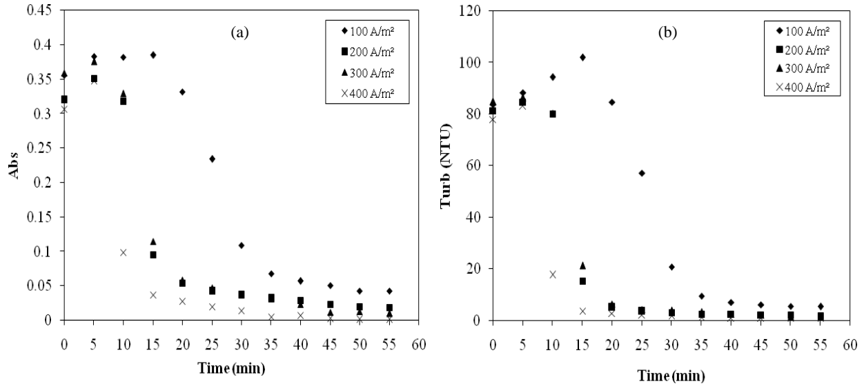
Fig. 3. Evolution of absorbance (a) and turbidity (b) during the treatment for different current densities j : C_0 = 50 \text{ mg L}^{-1} , initial pH 7.74, Q = 15 \text{ L h}^{-1} , e = 1 \text{ cm} , \kappa = 2.5 \text{ mS cm}^{-1}
