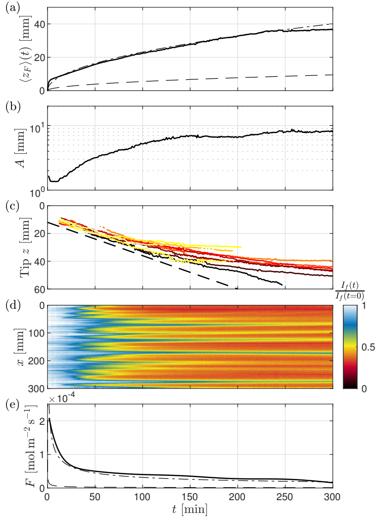
FIG. 4. Global measures of the instability. (a) Mean front depth \langle z_F \rangle as a function of time. The dashed line represents the expected diffusive front depth 2\sqrt{D_0 t} while the dashed dotted line highlights a diffusive behavior with a higher diffusion coefficient D_{\text{eff}} = 18D_0 . (b) Corrugation front amplitude A defined in Eq. (12) as a function of time t in a log-lin scale. (c) Fingertip depth (see Fig. 3(f) for an example of fingertip detection) as a function of time. Different colors are used to guide the eyes and easily follow the different fingertips. The dashed line shows a constant velocity of about 4 \times 10^{-3} mm/s for the fingertips at the beginning of the experiment. (d) Intensity profile at z = 15 mm as a function of time. White-blue regions correspond to low \text{CO}_2 concentrations and red/dark regions to high \text{CO}_2 concentration. (e) Temporal evolution of the \text{CO}_2 flux measured at the interface (solid line). The theoretical diffusive flux defined by Eq. (13) is plotted as a dashed line while the diffusive flux with a higher diffusion coefficient D_{\text{eff}} = 290D_0 is shown by a dashed dotted line. The initial \text{CO}_2 partial pressure is P_{\text{CO}_2}^0 = 0.6 bar and the thickness of the tank is 7 mm.
