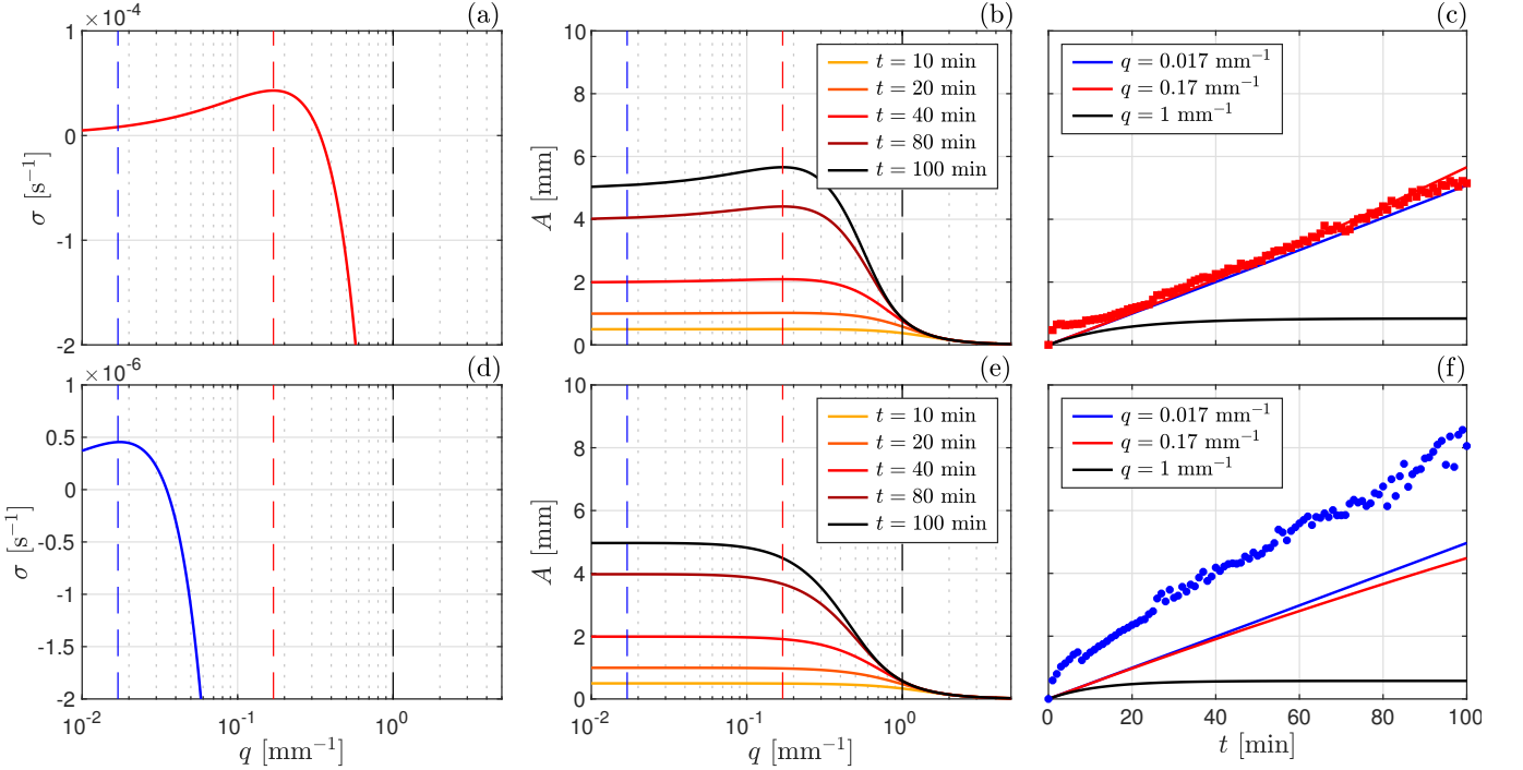
FIG. 8. Heuristic model for the growth of the front corrugation amplitude A as a function of time and wavenumber. The top line corresponds to an experiment at high \text{CO}_2 partial pressure ( P_{\text{CO}_2}^0 = 0.83 bar) while the bottom one is for an experiment at low \text{CO}_2 partial pressure ( P_{\text{CO}_2}^0 = 0.085 bar). These experiments are the same as the ones addressed in Figs. 5 and 6. The left column illustrates the dependence of the growth rate \sigma as a function of the wavenumber q using the heuristic model (28). The central and right columns show the evolution of the front corrugation amplitude A (given by Eq. (26) with \sigma(q) set by Eq. (28)) as a function of the horizontal wavenumber and time respectively. The colors of the vertical dashed lines marking different wavenumbers in the left and central columns correspond to the ones used in the right column. The experimental data, also shown in Fig. 5(c), are represented in panels (c) (red squares) and (f) (blue dots) as a reference.
