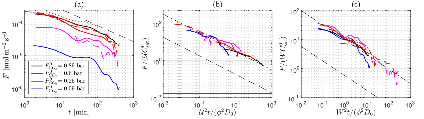
FIG. 9. CO 2 flux F as a function of time t for different initial CO 2 partial pressures P_{CO_2}^0 and different permeabilities. The experiments with FEP grains are represented with solid lines, while the ones with silica and PMMA grains are plotted with dashed and dashed dotted lines respectively. The data from the single experiment performed with fresh water and FEP grains is plotted as a red dotted line. The dimensional flux is shown in panel (a), while it has been made dimensionless in panels (b) and (c), using respectively \mathcal{F} = \mathcal{U}C_{\text{sat}}^0 and \mathcal{F}' = WC_{\text{sat}}^0 . The time t has also been made dimensionless, using \mathcal{T} = \phi^2 D_0 / \mathcal{U}^2 and \mathcal{T}' = \phi^2 D_0 / W^2 . The colors detailed in the legend in panel (a) are the same for all panels. In panel (b), the horizontal solid line indicates F/\mathcal{F} = 1.7 \times 10^{-2} , the expected dimensionless flux value for constant flux regime once the convection is well established [6, 7, 14, 20]. In panels (b) and (c), the dashed lines represent the expected dimensionless diffusive flux (see Eq. (32)) while the dashed dotted lines highlight a dimensionless diffusive flux with an effective diffusion coefficient D_{\text{eff}} = 290 D_0 .
