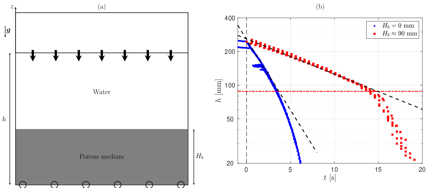
FIG. 10. (a) Sketch of the experimental setup to measure the permeability K of the porous medium. (b) Data obtained for the FEP grains: water level h as a function of time in a log-lin scale, without (blue dots) and with (red squares) grains at the bottom of the tank. The two dashed lines show the exponential fits to determine \gamma (fit of the blue dots) and K (fit of the red squares).
