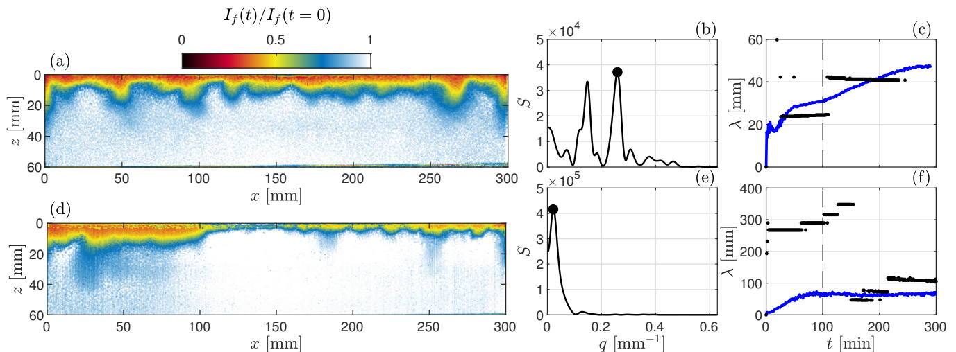
FIG. 6. Analysis of the front's dominant wavelength. (a) Snapshot at t = 100 min for an experiment at high \text{CO}_2 partial pressure ( P_{\text{CO}_2}^0 = 0.83 \text{ bar} ), shown in red in Fig. 5. (b) Spectrum S of the front for the image shown in panel (a). The maximum of the spectrum is indicated by a black dot. (c) Wavelength \lambda as a function of time determined using two different methods: the Fourier transform of the front (black dots) [24] and Eq. (27) (blue line) [7]. The vertical dashed line indicates the time of the snapshot shown in panel (a). (d), (e) and (f): Same panels as (a), (b) and (c) but for an experiment at low \text{CO}_2 partial pressure ( P_{\text{CO}_2}^0 = 0.085 \text{ bar} ), shown in blue in Fig. 5.
