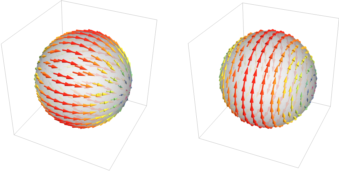
Figure 1: Real (left) and imaginary (right) parts of \delta_+(\xi) on the unit sphere |\xi| = 1 . Multiplication by a suitable prefactor in \mathbb{C} can rotate the axis (and the apparent singularity) of \delta_+(\xi) to any point on the sphere (the axis for the real and imaginary parts are the same). One obtains \delta_-(\xi) by complex conjugation of \delta_+(\xi) ; therefore, the imaginary part of the Fourier field “flows” the other way around in \mathbb{C}^3 .
