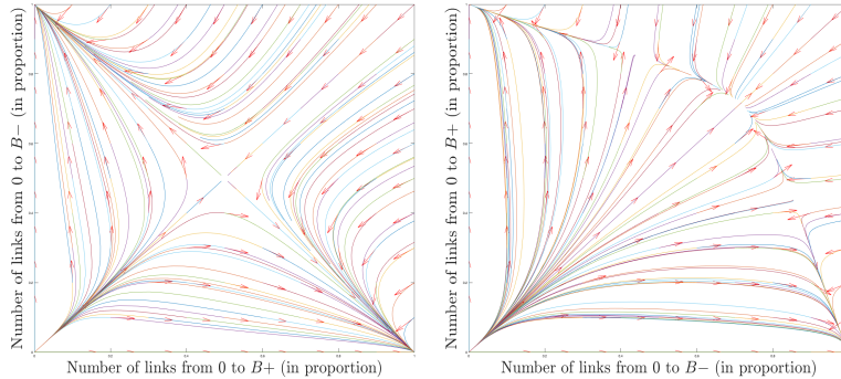
Figure 3: Phase portraits for the two cases \frac{\gamma}{\beta} = 2 (left) and \frac{\gamma}{\beta} = 3.5 . As expected, the symmetric equilibrium is stable and the 2 other equilibria are unstable in the later case.
