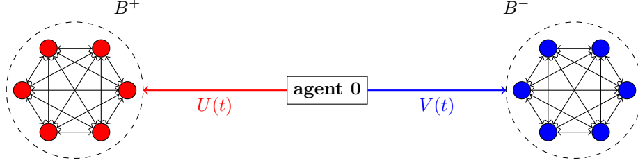
Figure 1: A single agent initially connected to two opposite stubborn cliques of same sizes |B^+| = |B^-| = 6 .
