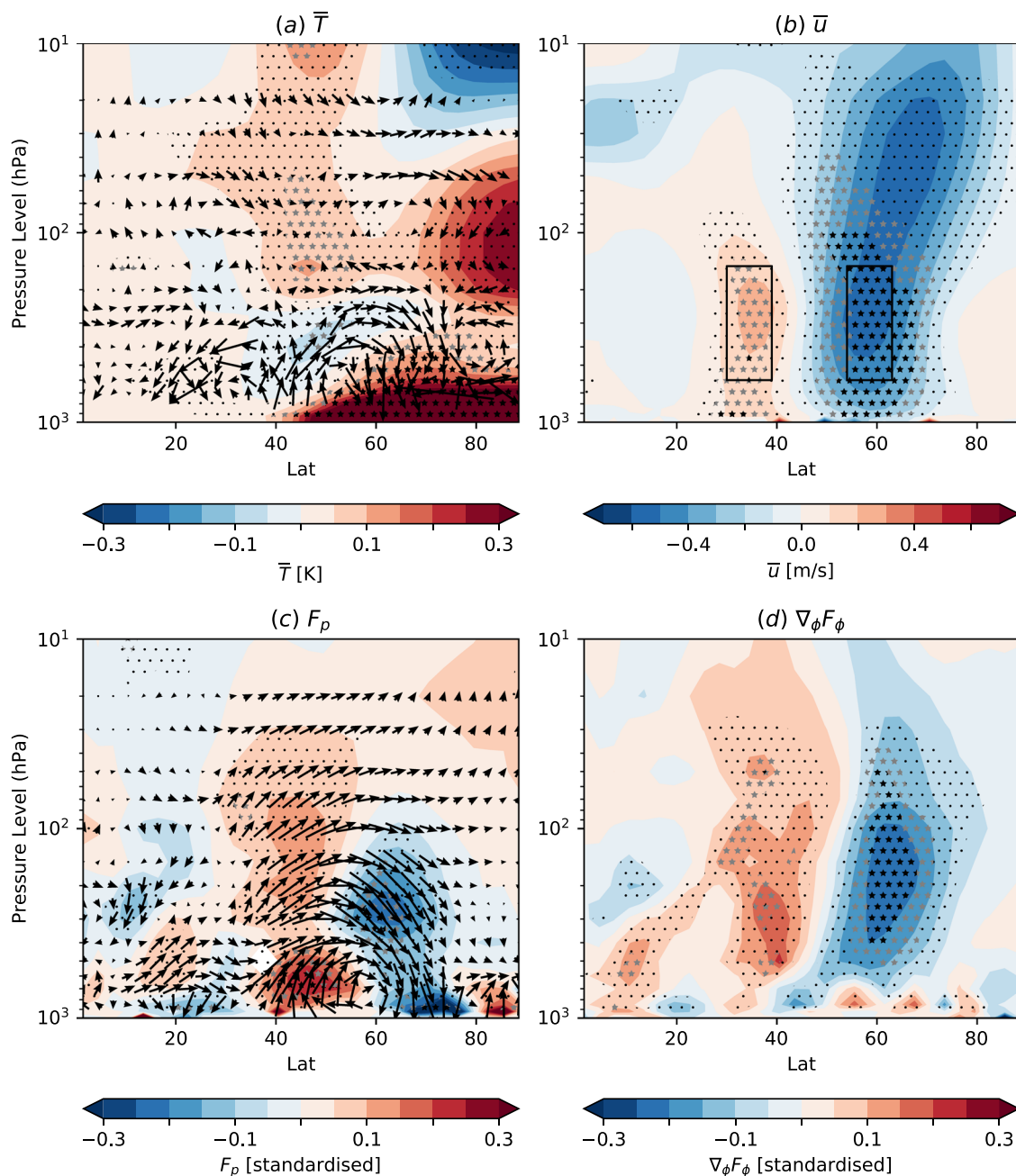
Fig. 3 Zonal mean response. Latitude-height cross sections of the multi-model ensemble mean zonal response of a temperature ( \bar{T} , colours, K, where the overbar denotes the zonal average) and transformed Eulerian mean (TEM, Methods) circulation (arrows), b zonal wind ( \bar{u} , \text{ms}^{-1} ), and c upward Eliassen-Palm (EP) flux ( F_p , colours, standard deviations) and EP flux vectors (arrows representing F_\phi and F_p ), d divergence of northward EP flux ( \nabla_\phi F_\phi , standard deviations). Stippling as in Fig. 1. To aid visualisation the TEM circulation and EP fluxes are standardised by dividing by the internal variability of the present-day simulations (Methods).
