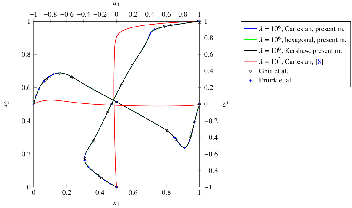
Figure 5: Two-dimensional lid-driven cavity flow with irrotational force \mathbf{f} = \lambda \nabla \psi with \lambda = 10^6 . Comparison between the present method and the original HHO formulation of [8] both using k = 1 . The plot represents the horizontal component u_1 of the velocity along the vertical centerline x_1 = \frac{1}{2} and the vertical component u_2 of the velocity along the horizontal centerline x_2 = \frac{1}{2} for \text{Re} = 1,000 .
