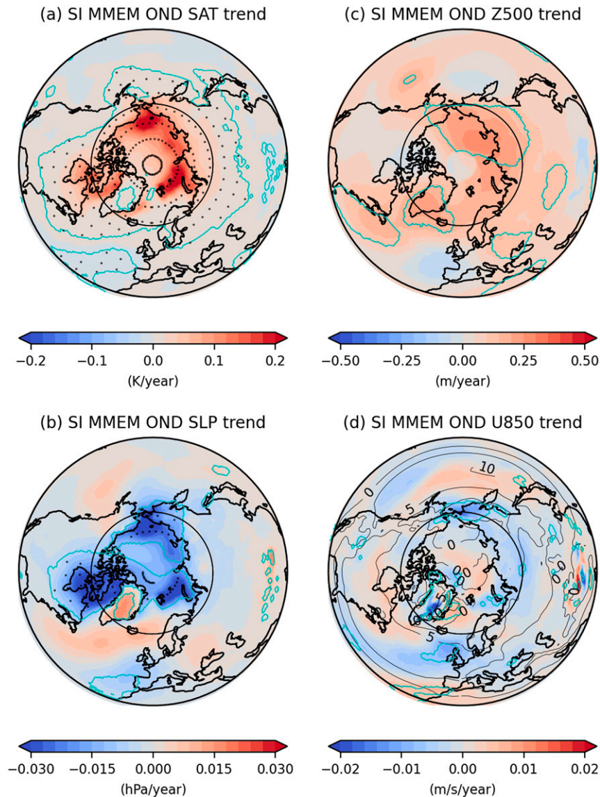
FIG. 6. OND trends from SI MEMM for (a) SAT, (b) SLP, (c) geopotential height at 500-hPa level (Z500), and (d) zonal wind at 850-hPa level (U850). The cyan contour lines indicate the 5% local significance level, while the black dots denote the field significance. The black contour lines in (d) represent climatological (1979–2014) OND ALL MEMM U850 (in \text{m s}^{-1} ). The 165 members are used in (a) and (b), while 155 members are used in (c) and (d).
