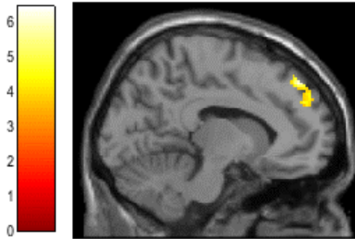
Figure 8. Final (incorrect) conflict trials – final (correct) non-conflict trials.
