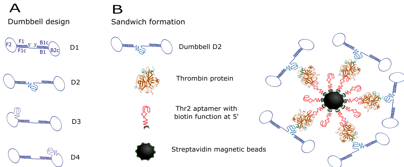
Figure 1: (A) Scheme of the different dumbbell designs. D1 is the minimal dumbbell construct and does not contain any aptamer sequence. D2, D3 and D4 present the aptamer in various positions. (B) Scheme of the double aptamer sandwich formation for the capture of thrombin prior to the isothermal dumbbell exponential amplification. Magnetic beads functionalized with Thr2 aptamer were used to capture the target, thrombin protein, and the dumbbell structure incorporating the Thr1 aptamer was used as a recognition probe. After proper rinsing of the non-reacted dumbbells, the remaining ones were then put in contact with a LAMP reaction mix and warmed at 65°C during 60 minutes for an exponential isothermal amplification and further quantification.
