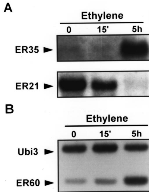
Fig 3. Ethylene-regulated expression of cloned cDNAs. (A) Northern blot analysis of positive clones ER21 and ER35. Northern blots were carried out using 25 \mu g of total RNA from untreated fruit (0) and from fruit treated with ethylene for 15 min (15') or 5 hours (5 h). (B) RT-PCR detection of ER60 expression. Total RNA from untreated fruit (0) and from fruit treated with ethylene for 15 min (15') or 5 hours (5 h) were reverse transcribed in the presence of an oligo-d(T)21 primer. The PCR amplification was performed using ER60 cDNA specific primers. As an internal control, the endogenous tomato ubiquitin cDNA (Ubi3) was amplified concomitantly with ER60 by adding to the PCR reaction Ubi3 specific primers. The PCR products were separated on a 1.4% agarose gel, transferred to a nylon membrane and hybridized with a mixture of equal cpm of ER60 and Ubi3 probes. The membranes were exposed to Amersham Hyperfilm-MP at -80^{\circ}\text{C} for 60 min.
