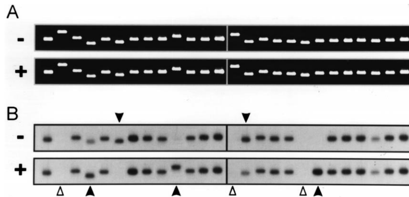
Fig 1. Elimination of false positive bands prior to cloning. (A) Differential bands eluted from the polyacrylamide gel were re-amplified. Equal amounts of the reamplified fragments were run in duplicate (- and +) on the same agarose gel and displayed following ethidium bromide staining. (B) Reverse Northern screening. The cDNA fragments were transferred onto a Nylon membrane. The duplicate membranes were then hybridized overnight, one to a total cDNA probe from ethylene treated tomato fruit (+), and the other to a total cDNA probe from the untreated sample (-). The closed arrowheads indicate differential bands and open arrowheads show bands with no expression signal.
