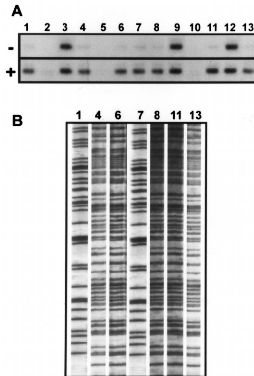
Fig 2. Selection of colonies containing differentially-expressed inserts. (A) Elimination of constitutively expressed cDNAs contaminating the cloned fragments. Fragments showing a differential signal in Fig. 1 were cloned and the cDNA inserts corresponding to one DD band were PCR-amplified from single colonies. The PCR products were then processed for analysis by reverse Northern as indicated in Fig. 1. (B) Identification of independent sequences by partial sequencing. The partial DNA sequencing of the true differential clones (colonies 1, 4, 6, 7, 8, 11, 13) was performed using the colony lysates directly as a source of DNA template. The patterns represent the sequencing reactions performed with only ddGTP in the termination step.
