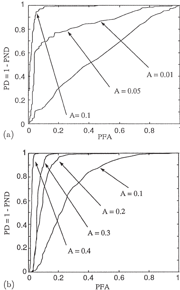
Fig. 9. ROC curves for the GLRD: (a) white noise, (b) colored noise.
