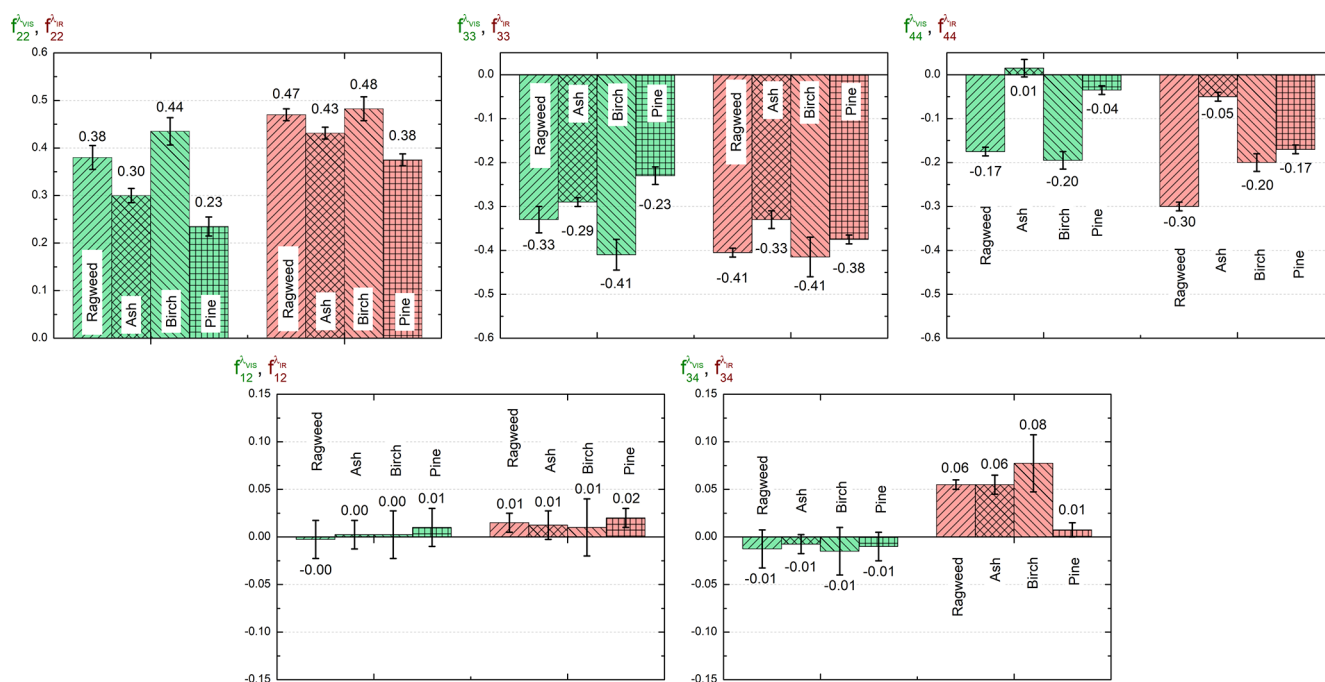
Figure 5. Retrieved scattering matrix elements of ragweed, ash, birch and pine at a 177.5^\circ scattering angle at wavelengths \lambda_{\text{VIS}} and \lambda_{\text{IR}} , with corresponding uncertainties evaluated by applying the methodology presented in Sect. 3. For each pollen taxon, the evaluation of the scattering matrix has been repeated with different samples: each evaluated scattering matrix lies within presented error bars.
